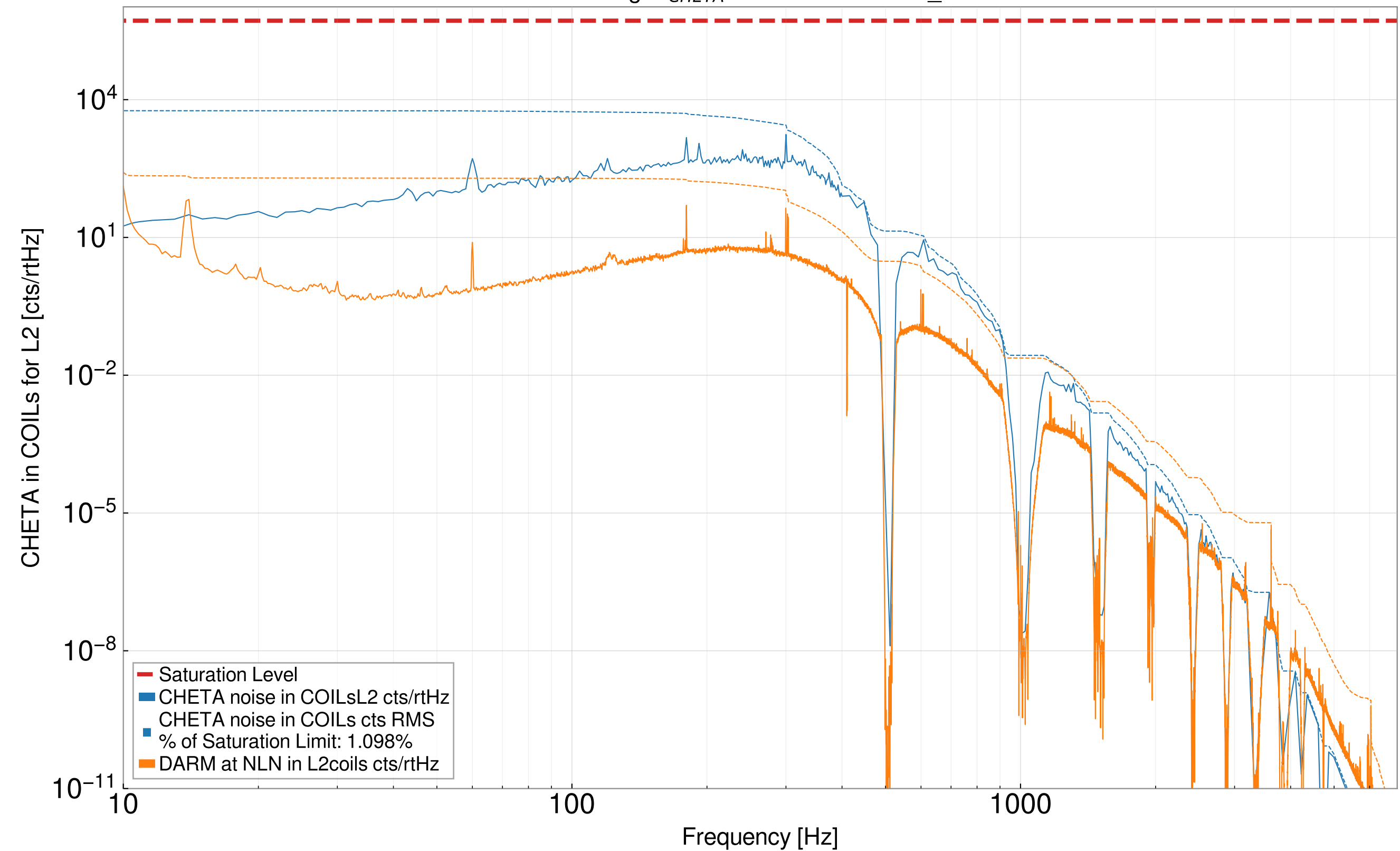
Calibrating \delta I_{CHETA} to counts before L2_DAC
