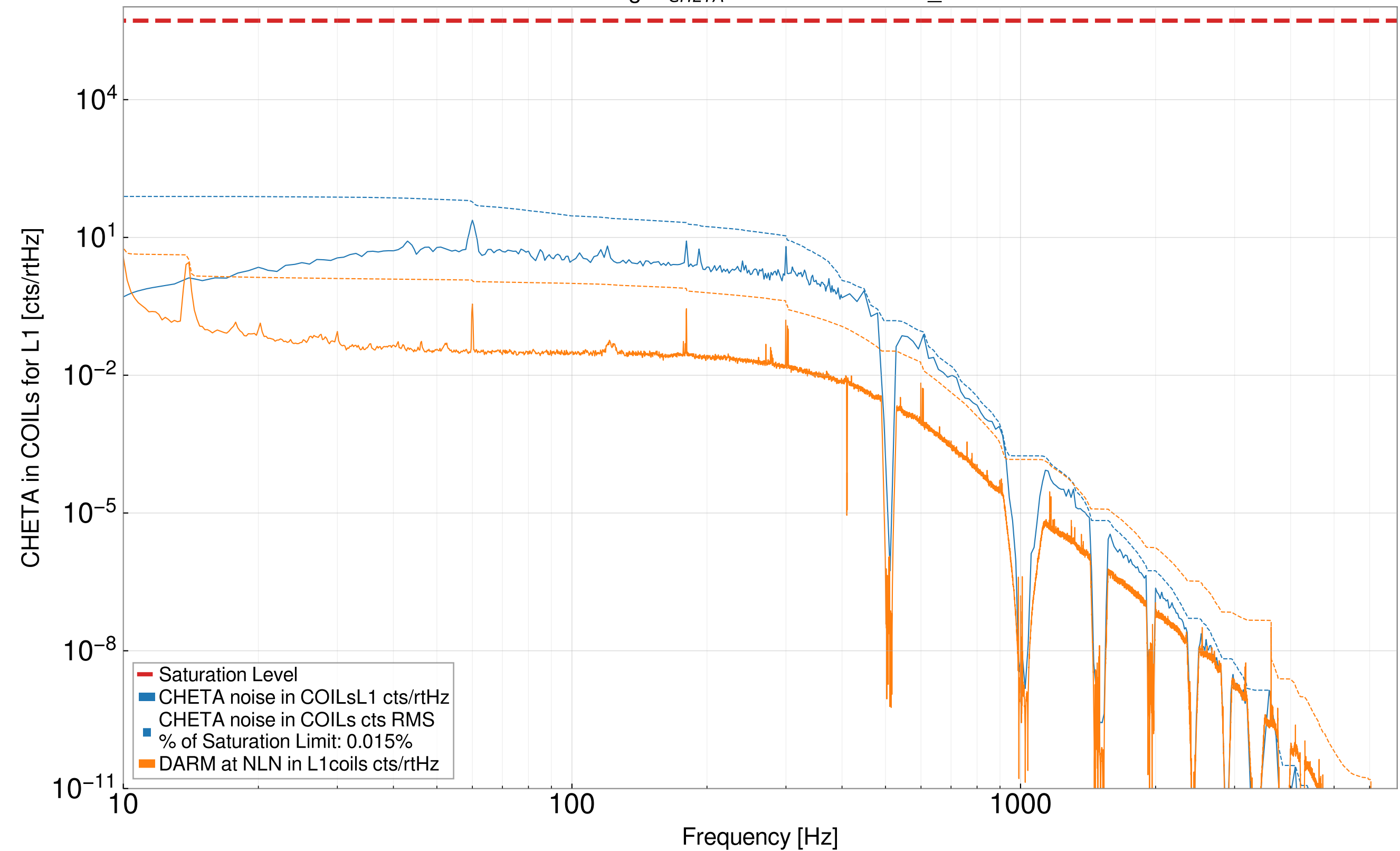
Calibrating \delta I_{CHETA} to counts before L1_DAC
