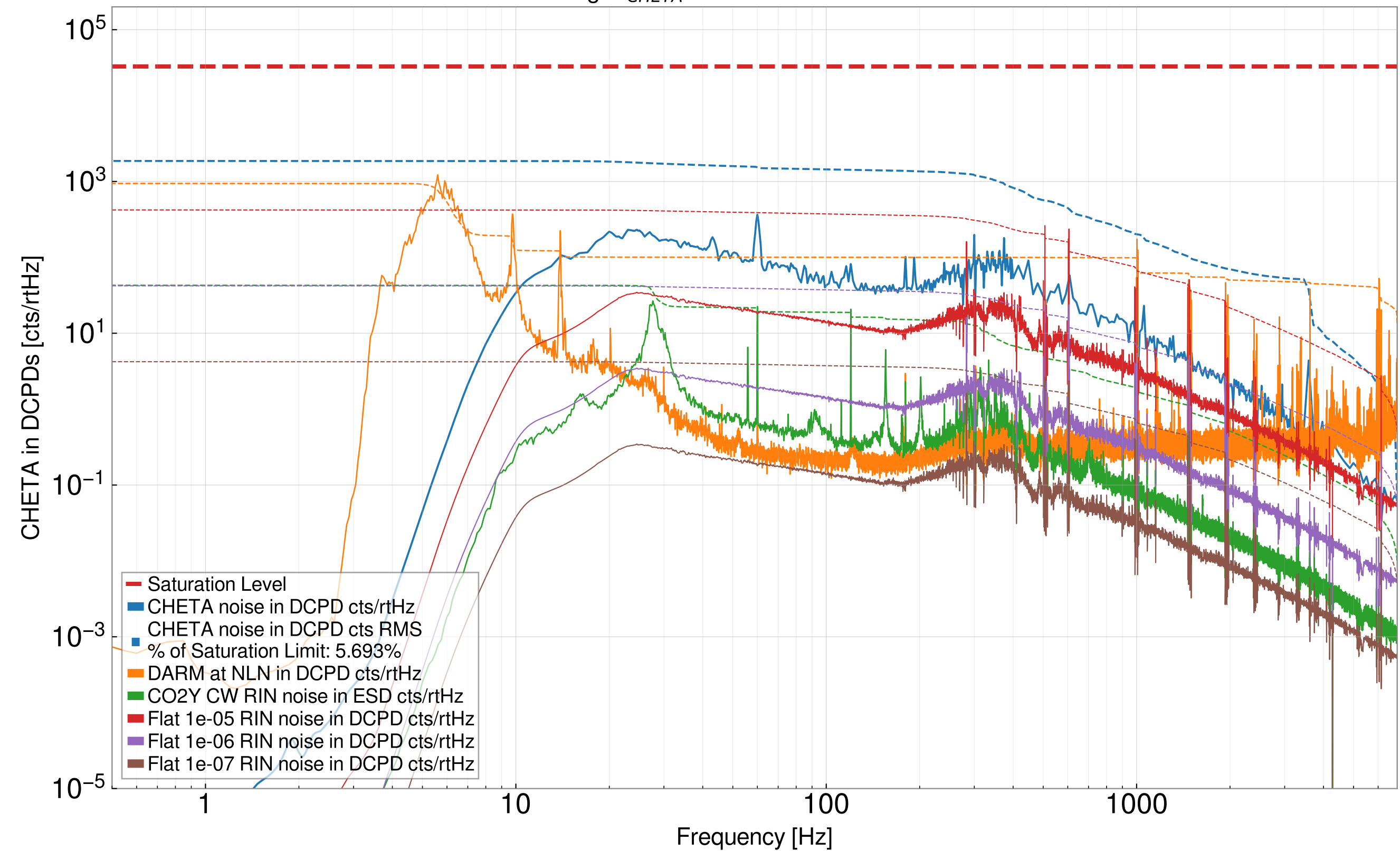
Calibrating \delta I_{CHETA} to counts before DCPD : P = 1W
