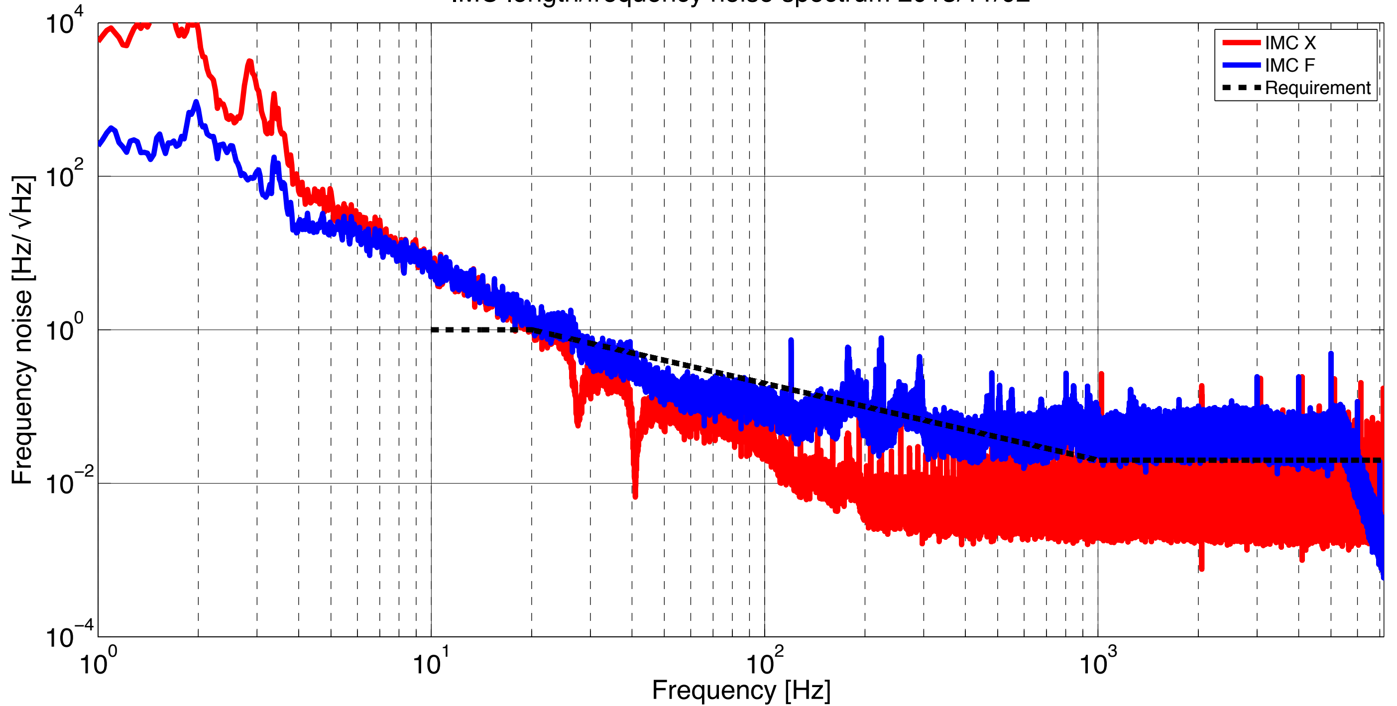
IMC length/frequency noise spectrum 2013/11/02
