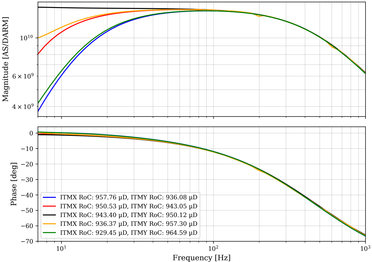
DARM input->DARM readout at Differential ITM RoC
