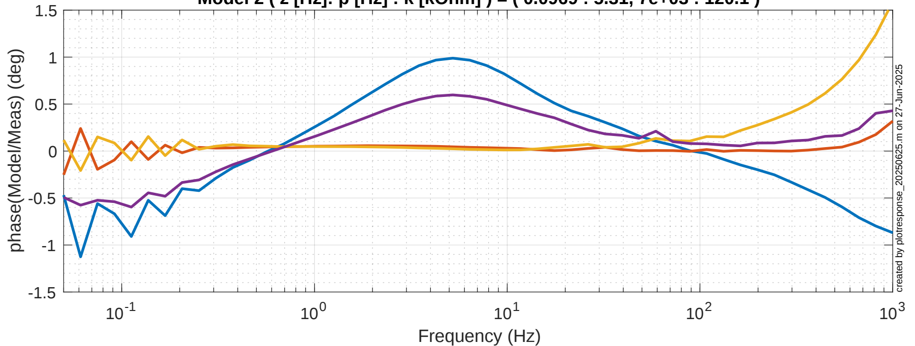
Model 2 ( z [Hz]: p [Hz] : k [kOhm] ) = ( 0.0969 : 5.31, 7e+03 : 120.1 )
