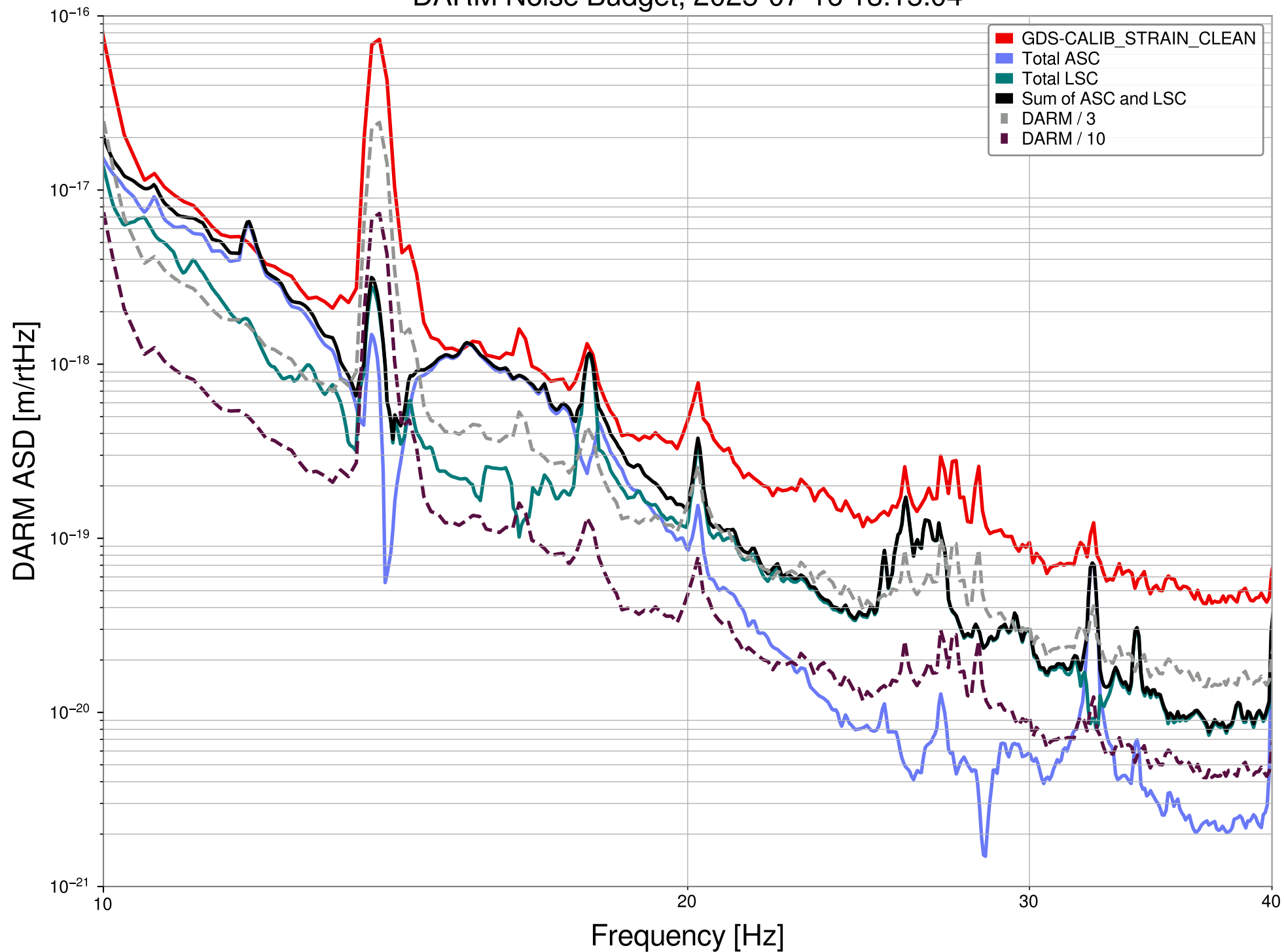
DARM Noise Budget, 2025-07-16 13:15:04
