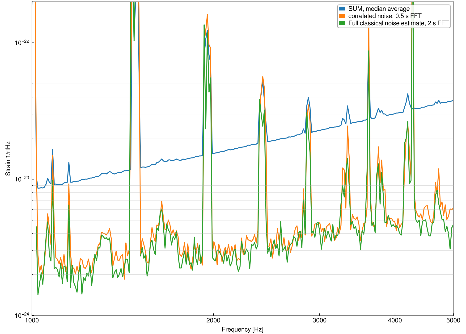
Correlated Noise
