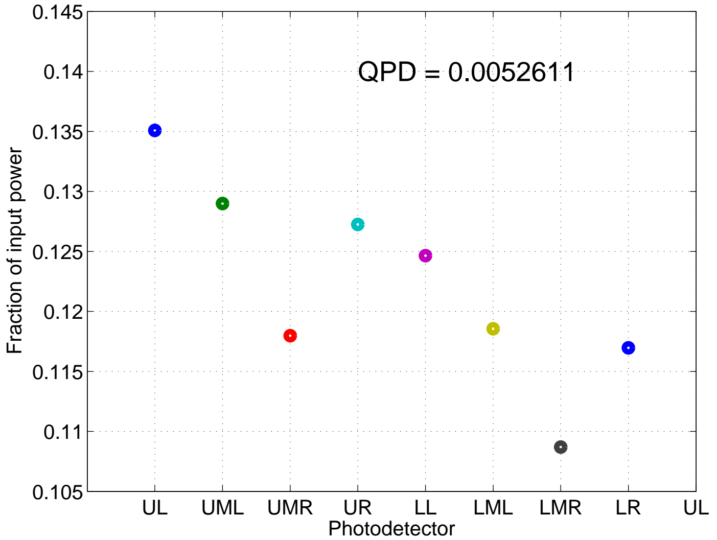
H1 ISS PD array relative powers on PDs, Nov. 7, 2013
