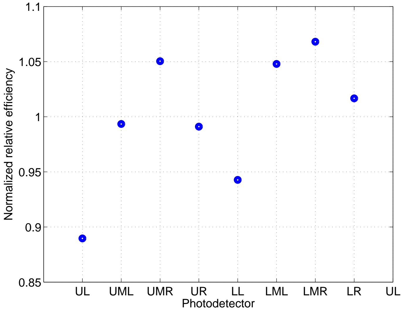
DC voltage divided by fractional power (normalized to mean)
