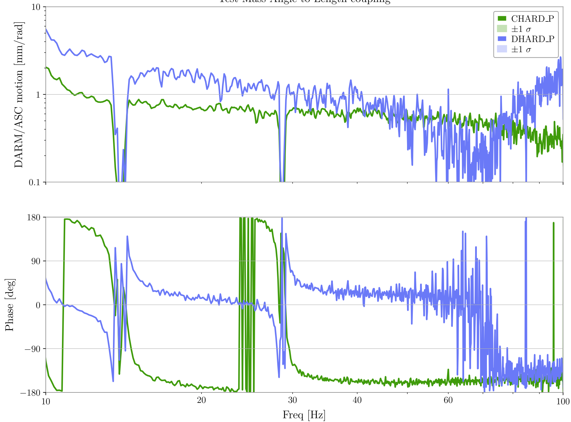
Test Mass Angle to Length coupling
