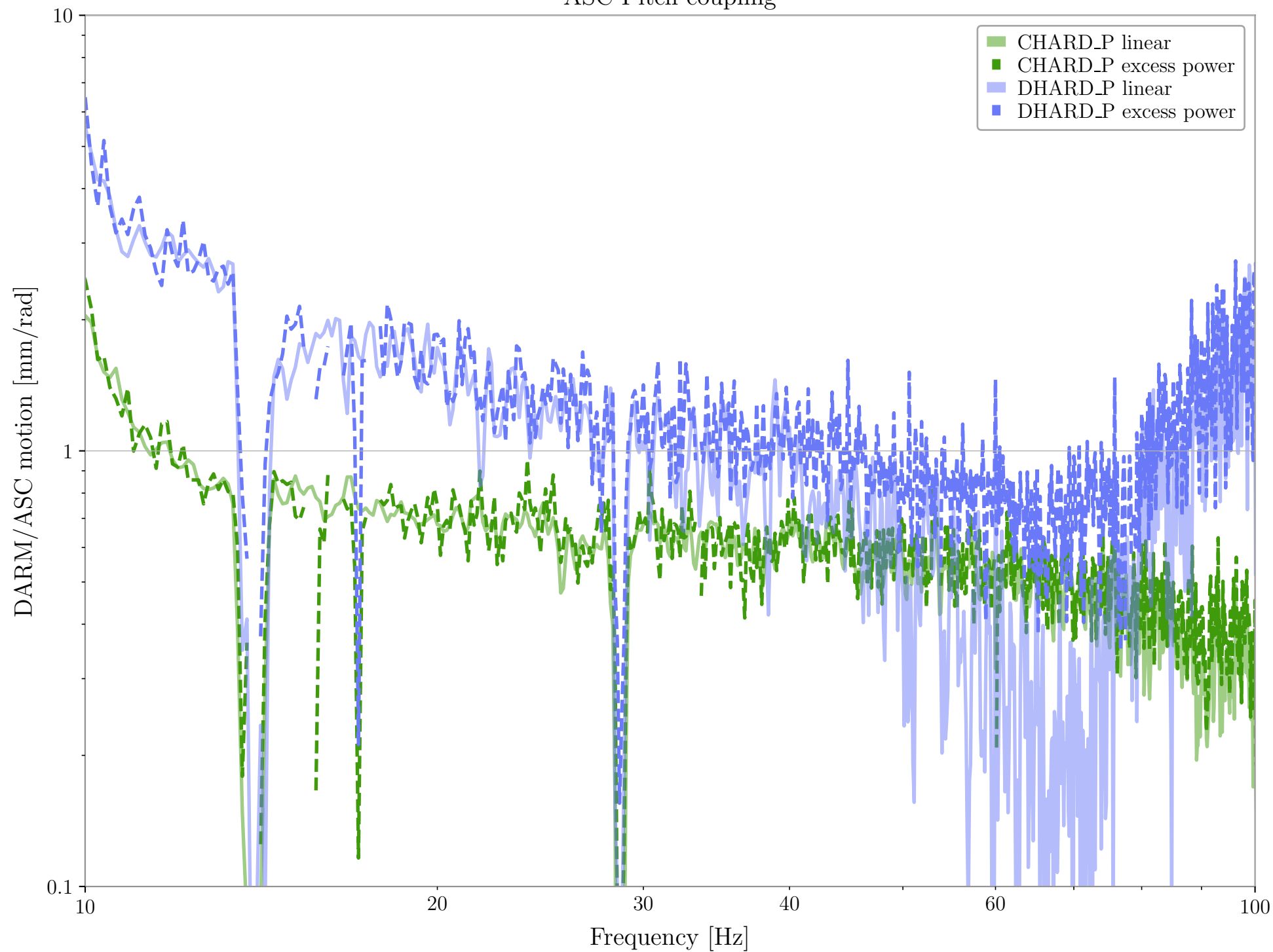
ASC Pitch coupling
