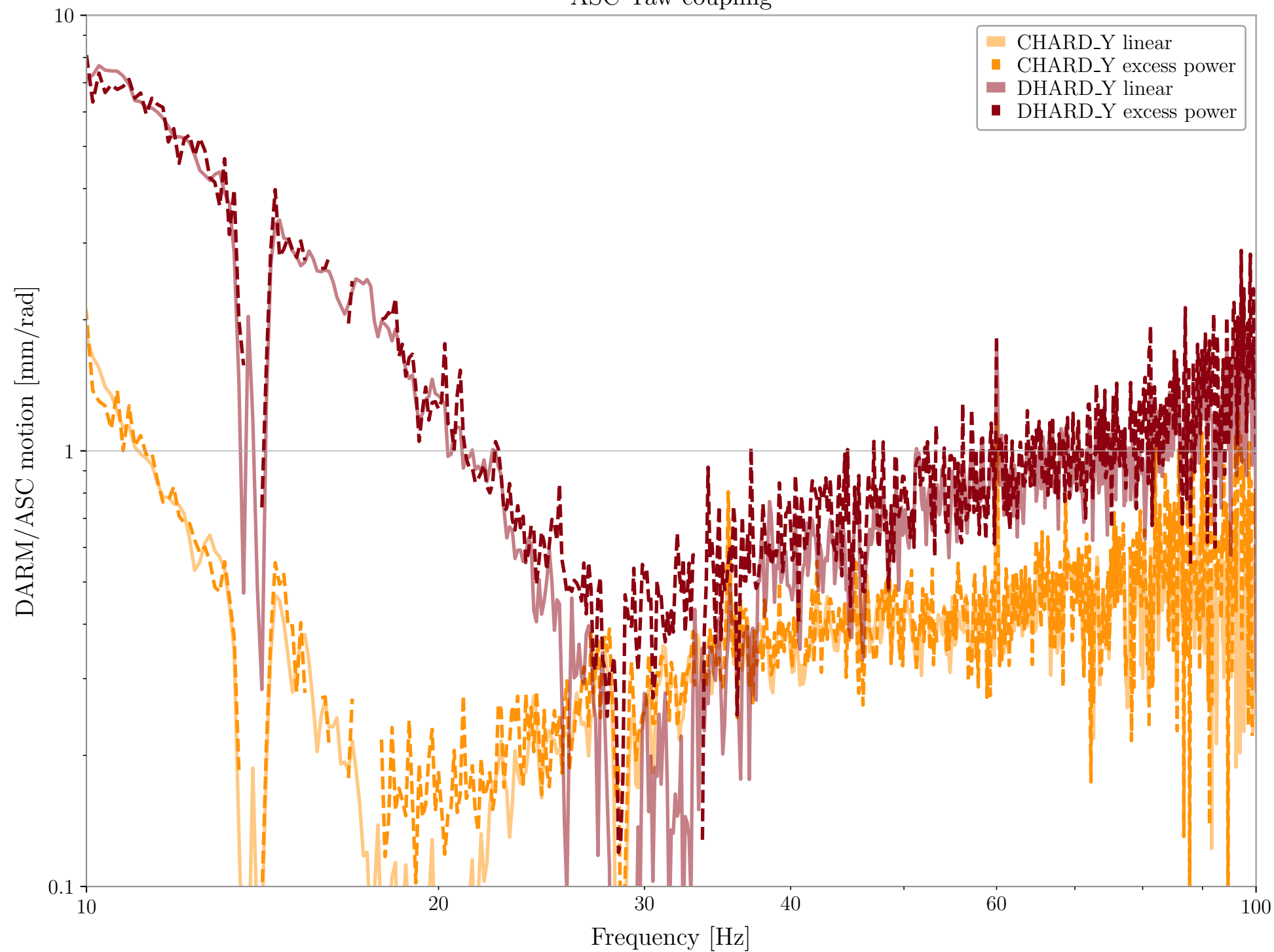
ASC Yaw coupling
