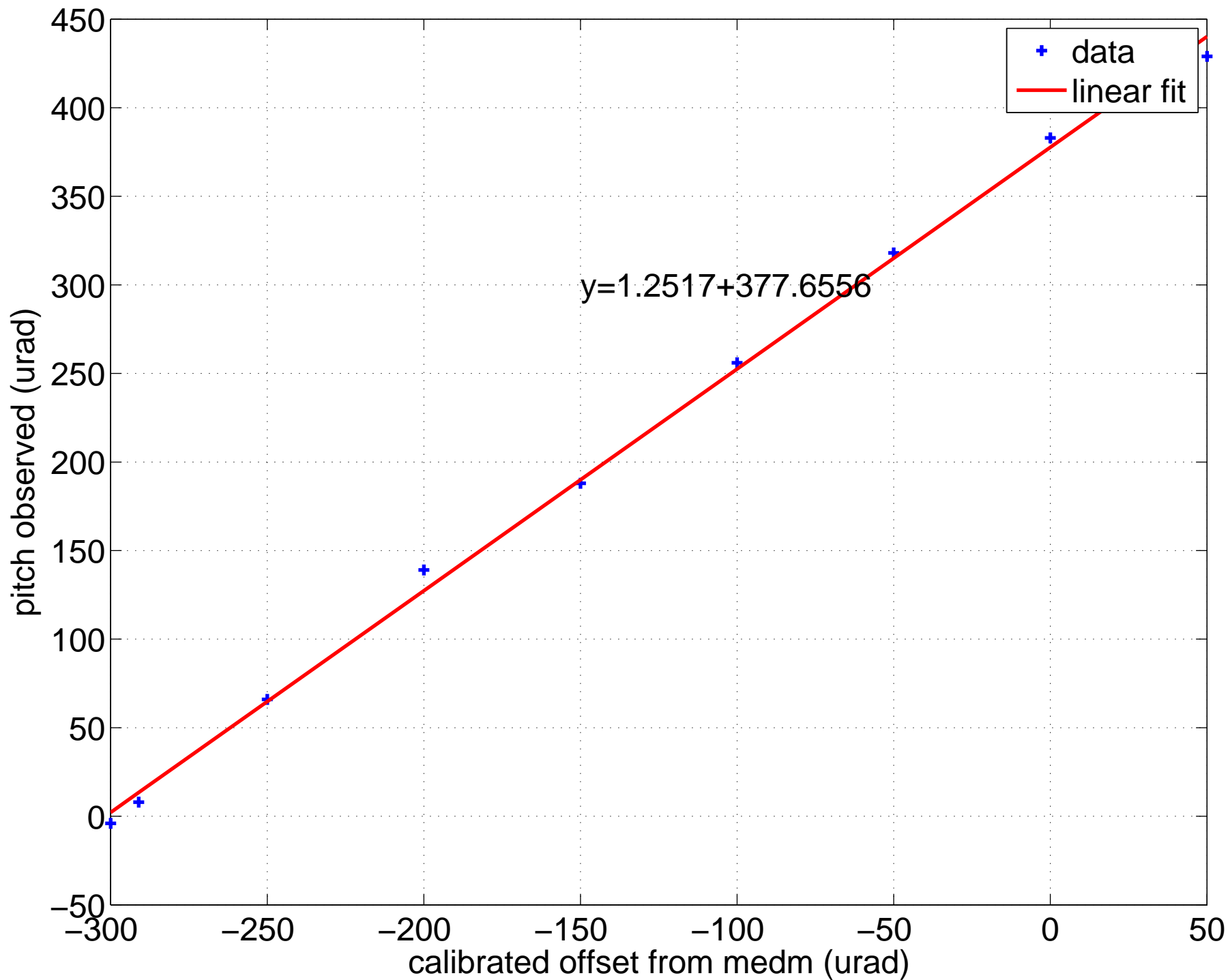
Test mass pitch calibration
