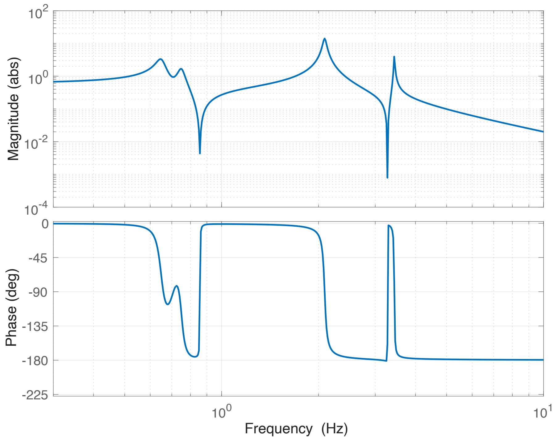
SR3 Fit, M1 drive P to M1 OSEM P
