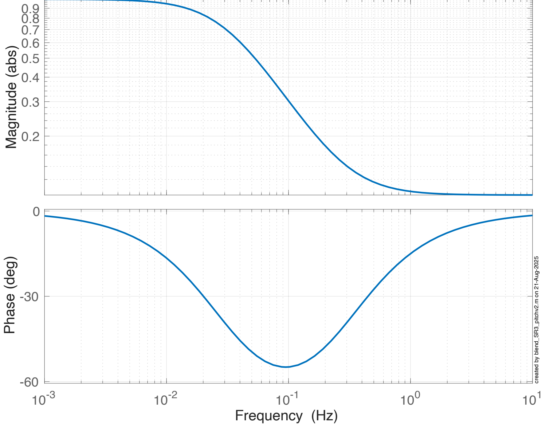
Bode Diagram
