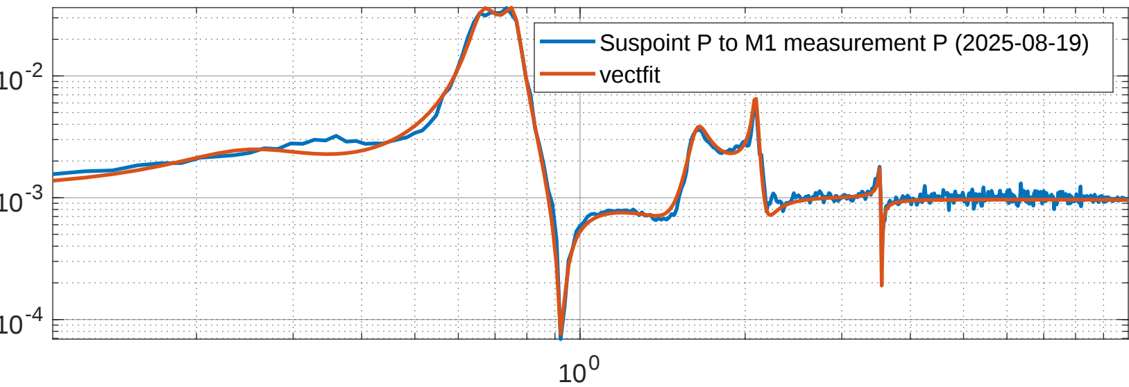
PR3 Suspoint P to M1 P (vectfit3)
