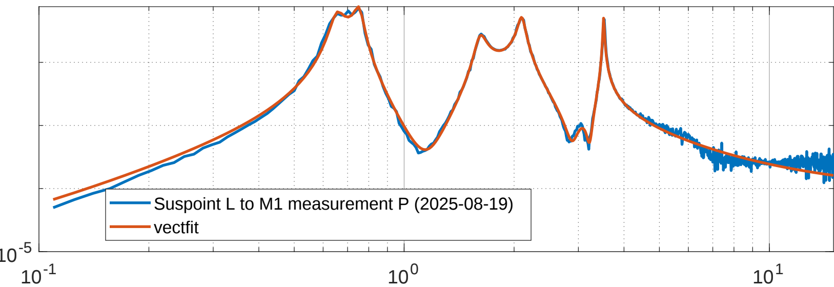
PR3 Suspoint L to M1 P (vectfit3)
