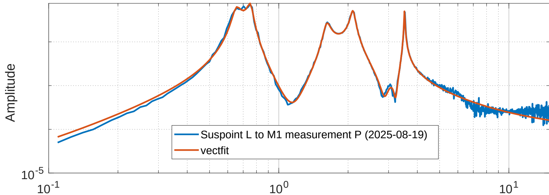
PR3 Suspoint L to M1 P (vectfit3)
