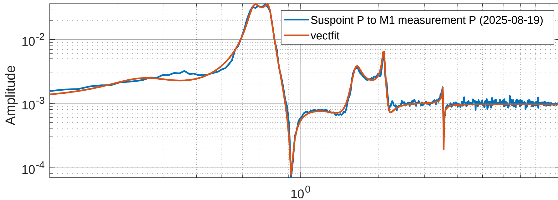
PR3 Suspoint P to M1 P (vectfit3)
