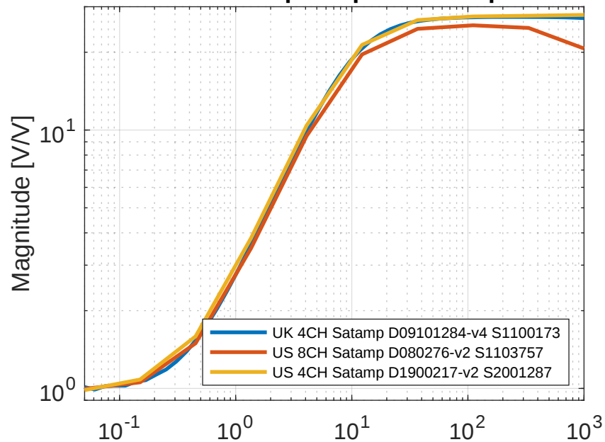
OSEM PD Satamp Response Comparison
