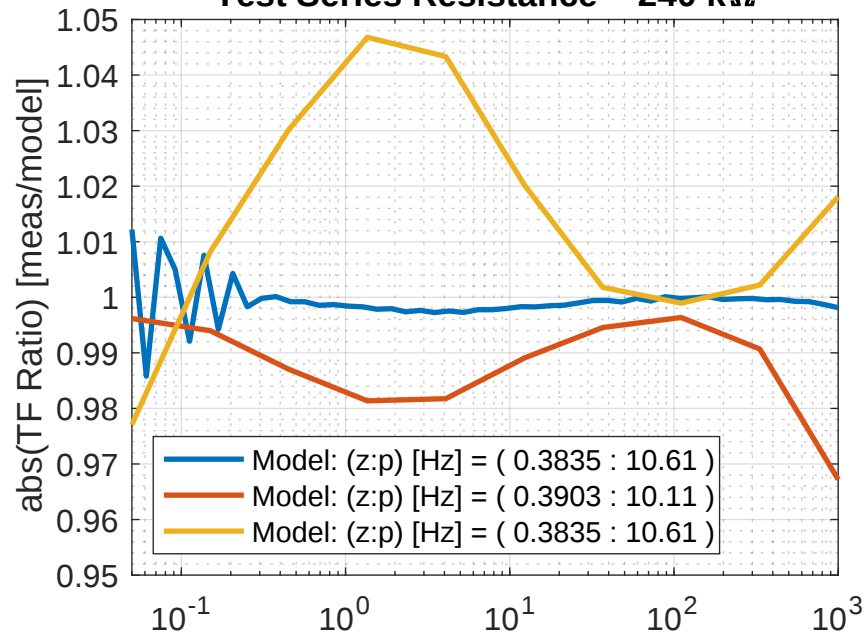
Test Series Resistance ~ 240 k \Omega
