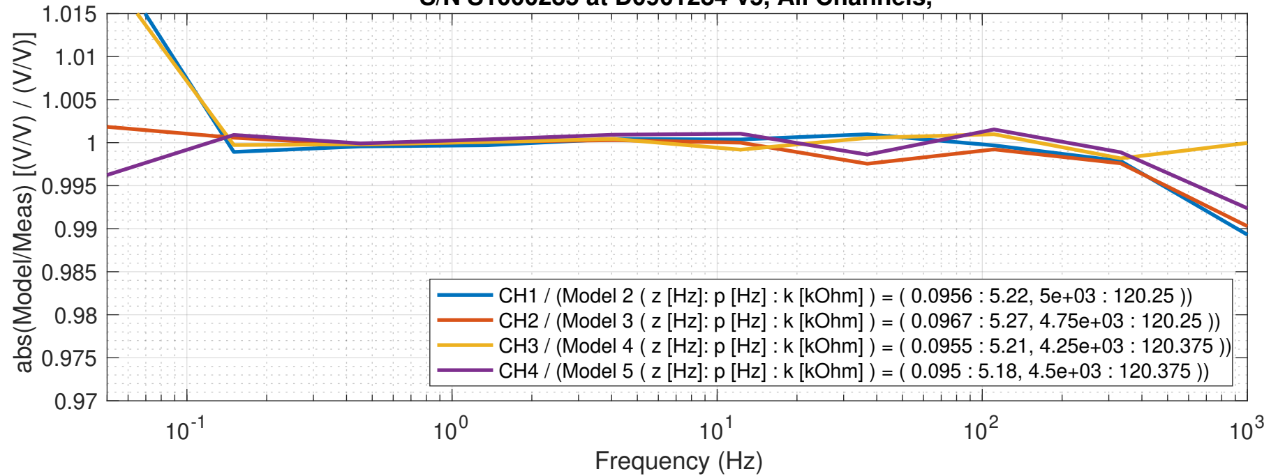
S/N S1000285 at D0901284-v5, All Channels,
