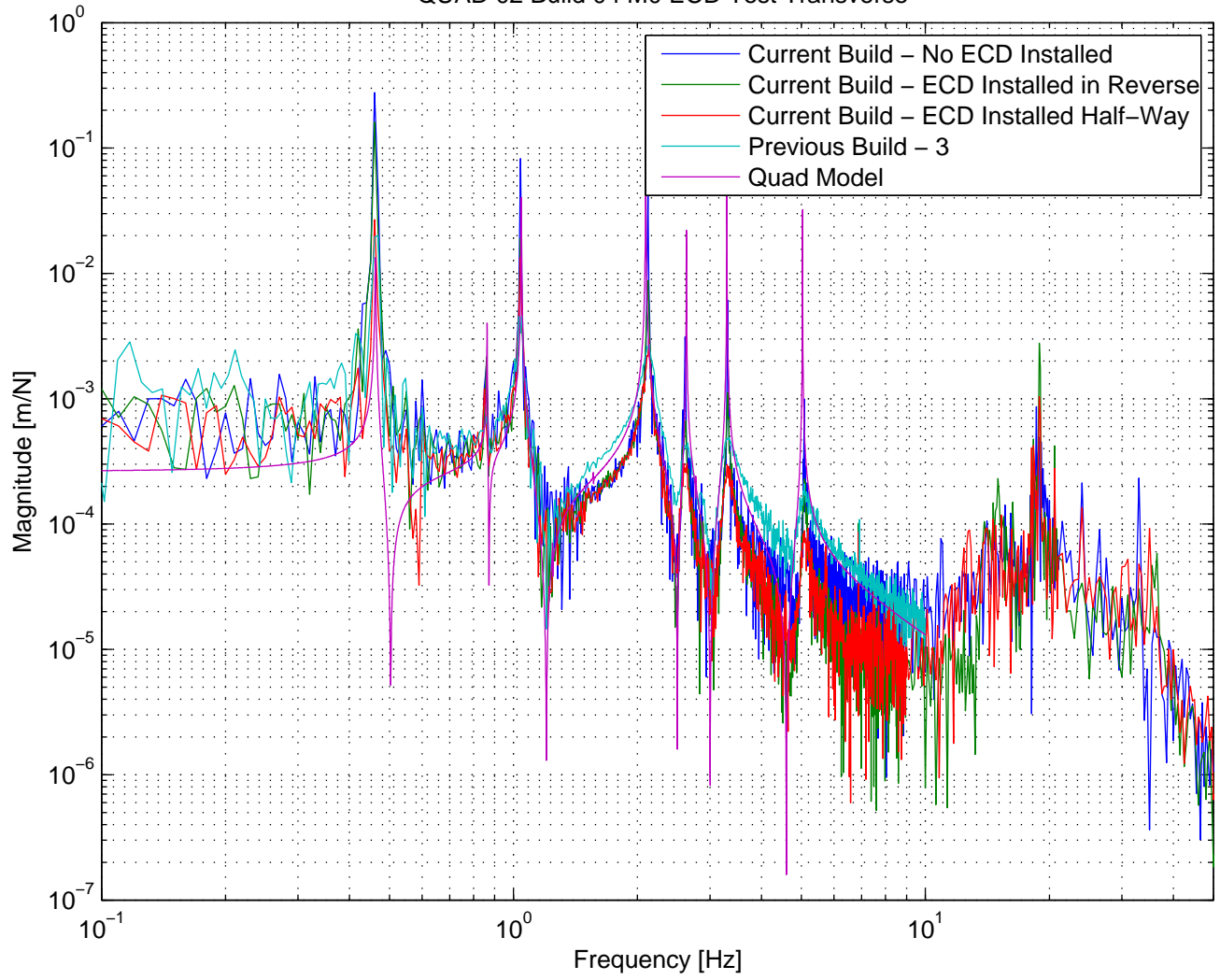
QUAD 02 Build 04 M0 ECD Test Transverse
