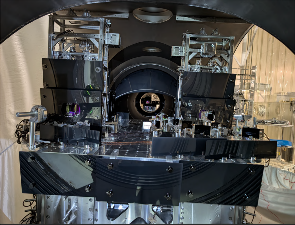
Baffles on the +X side of HAM3
