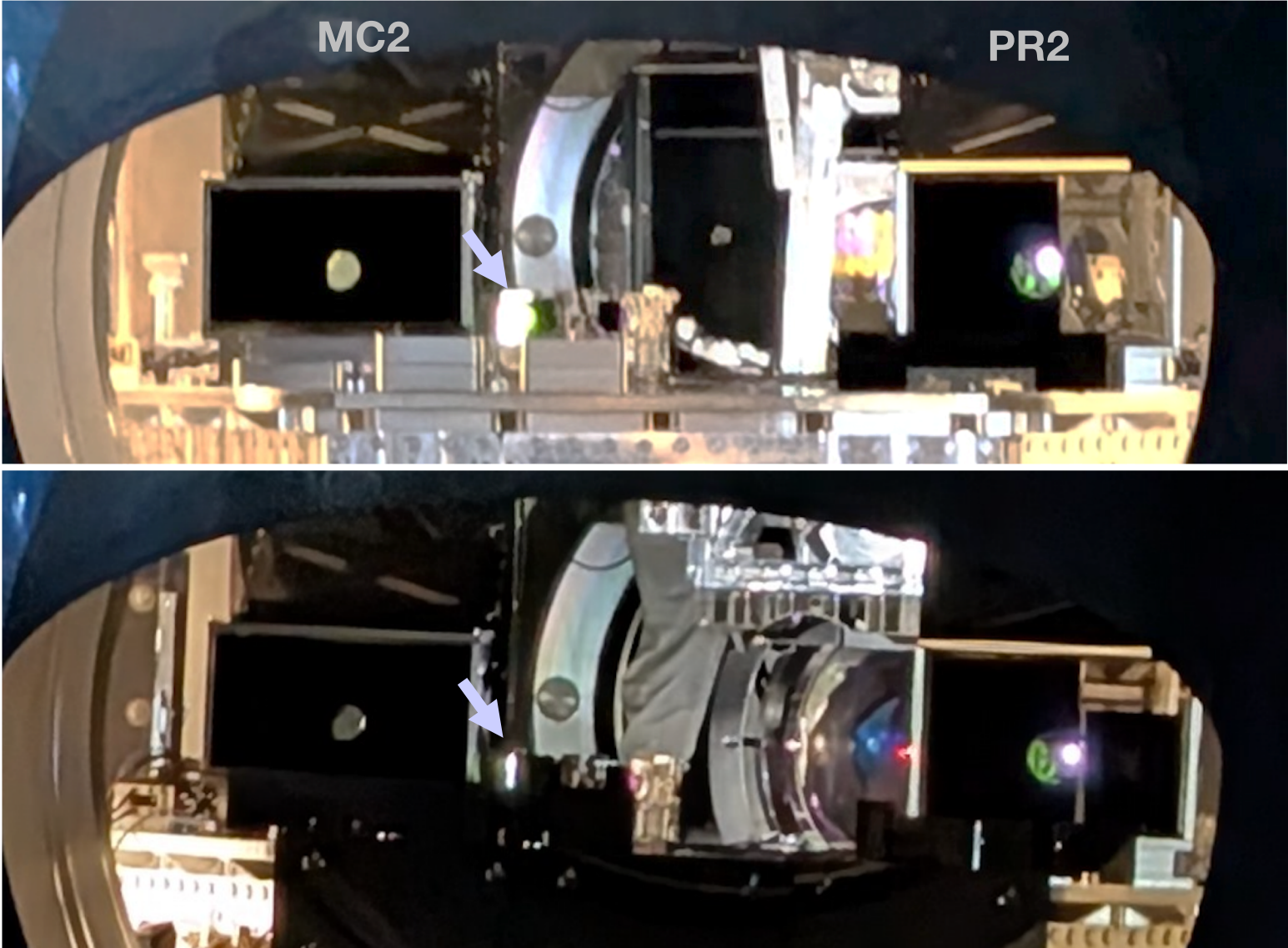
View of HAM3 from PRM before and after baffling and fix of direct reflection of PRM scattered light from POP optic (arrow)
