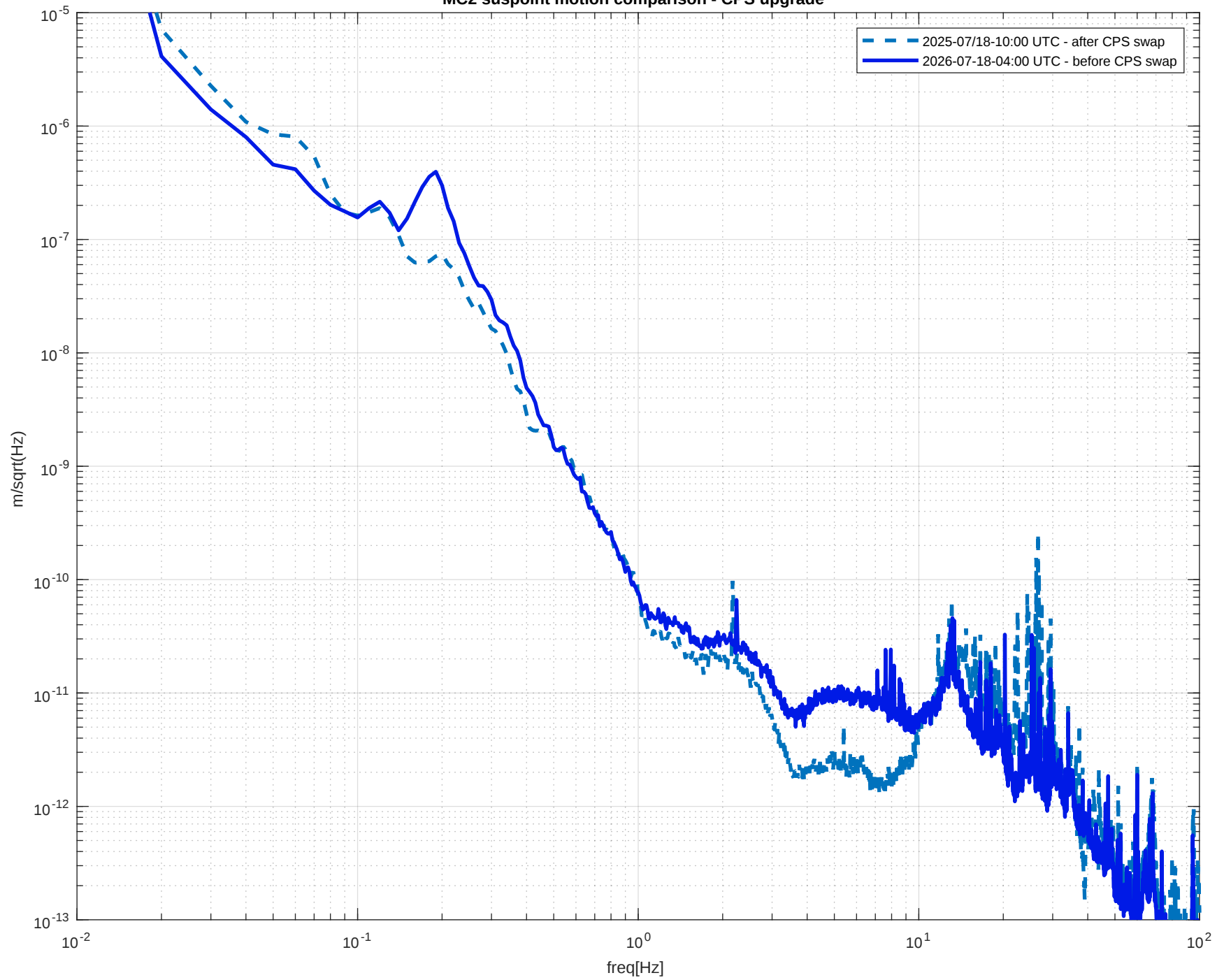
MC2 suspoint motion comparison - CPS upgrade
