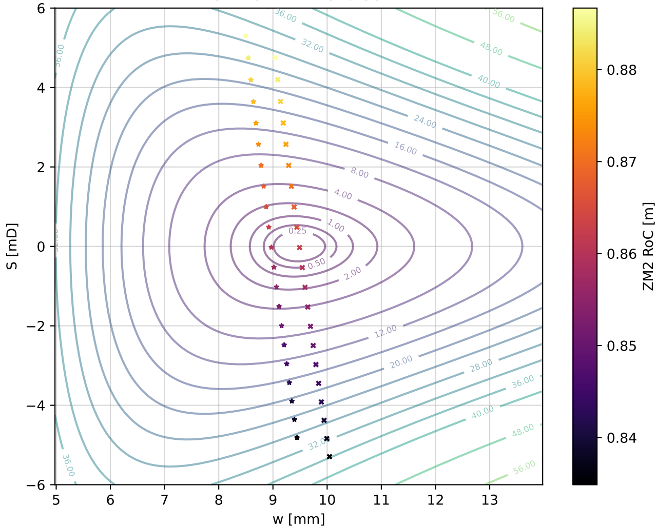
FC1 w-S space vs. PSAMs power Nominal ZM2 Rc: 0.86m
