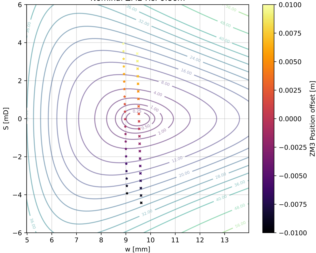
FC1 w-S space vs. ZM3 Position Nominal ZM2 Rc: 0.86m
