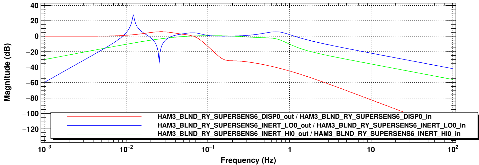
Transfer function
