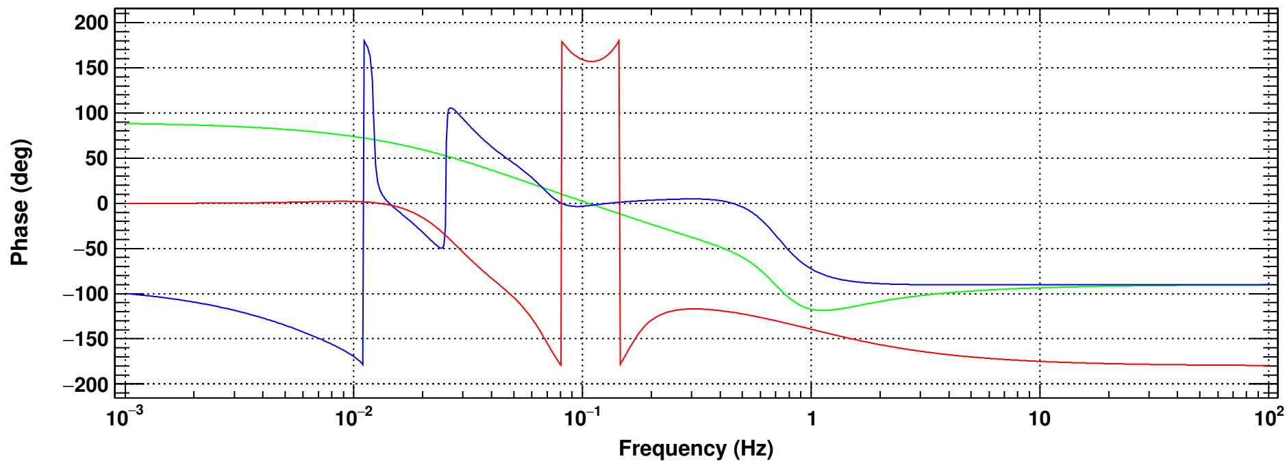
Transfer function
