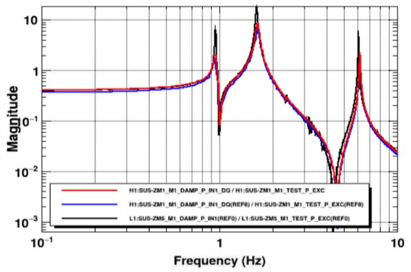
Transfer function
