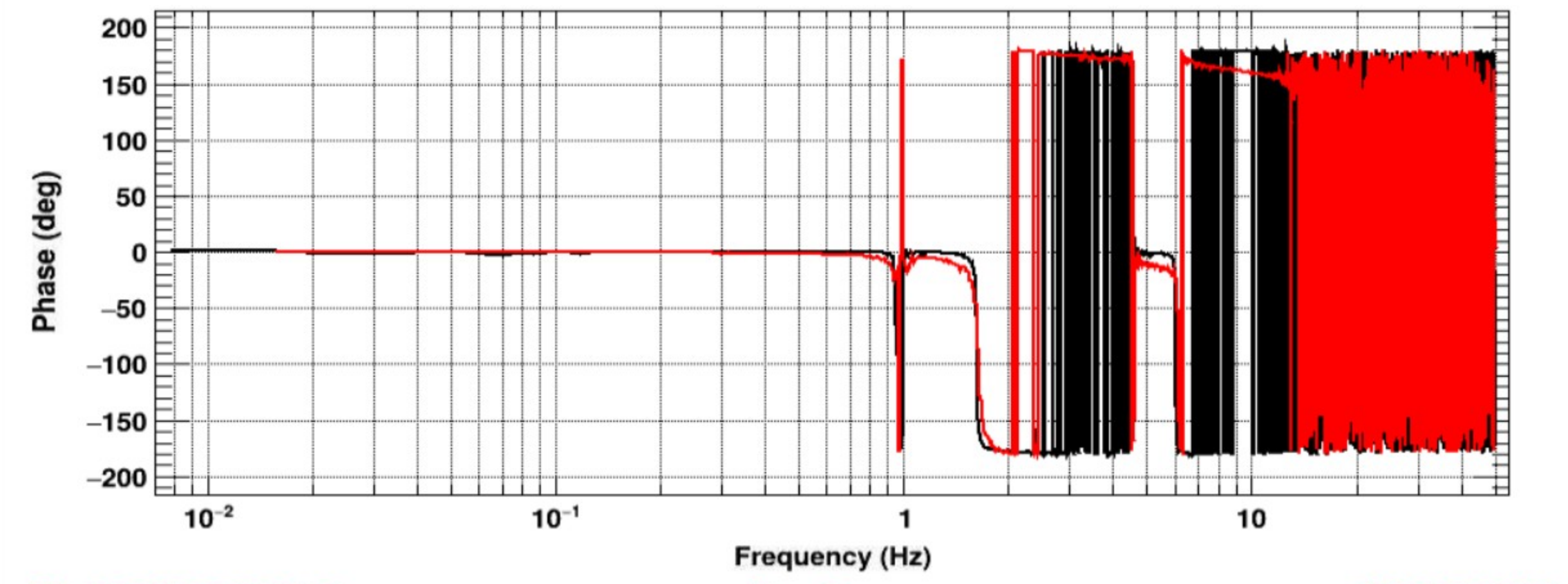
Transfer function
