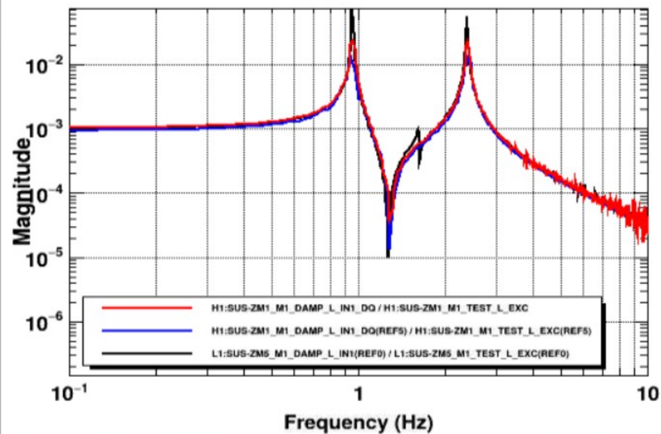
Transfer function
