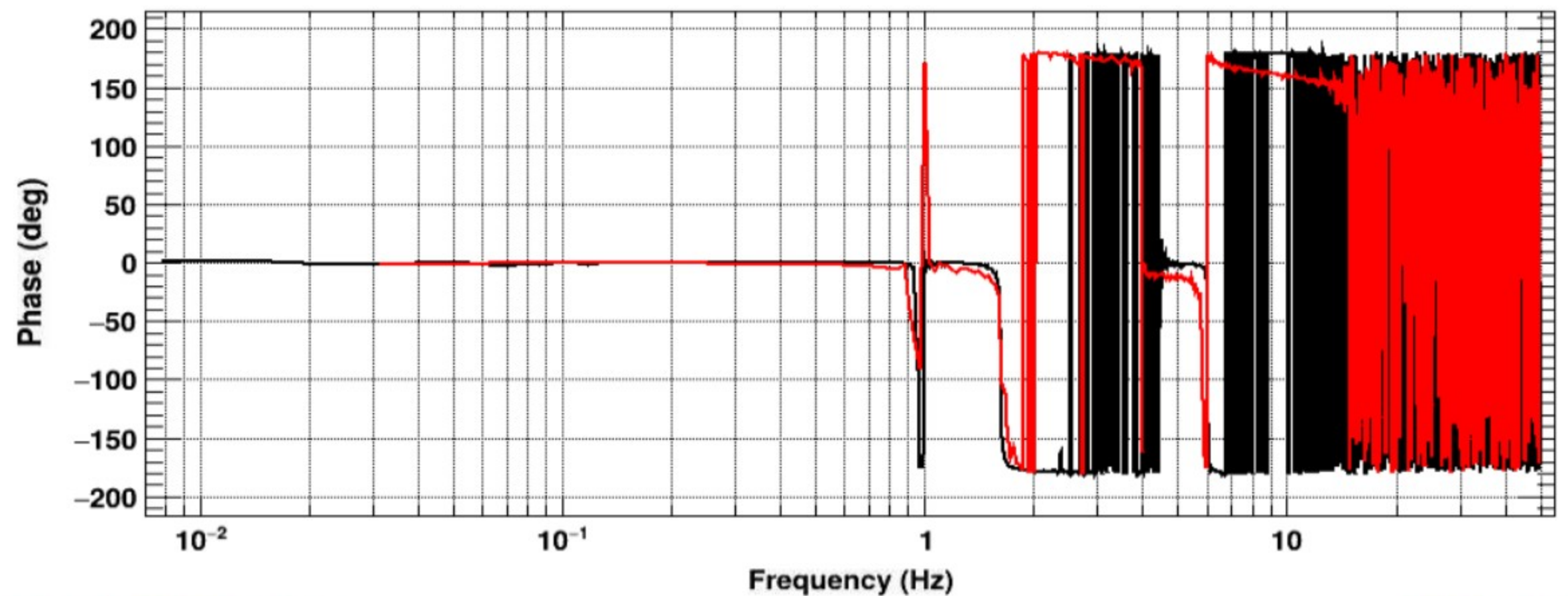
Transfer function
