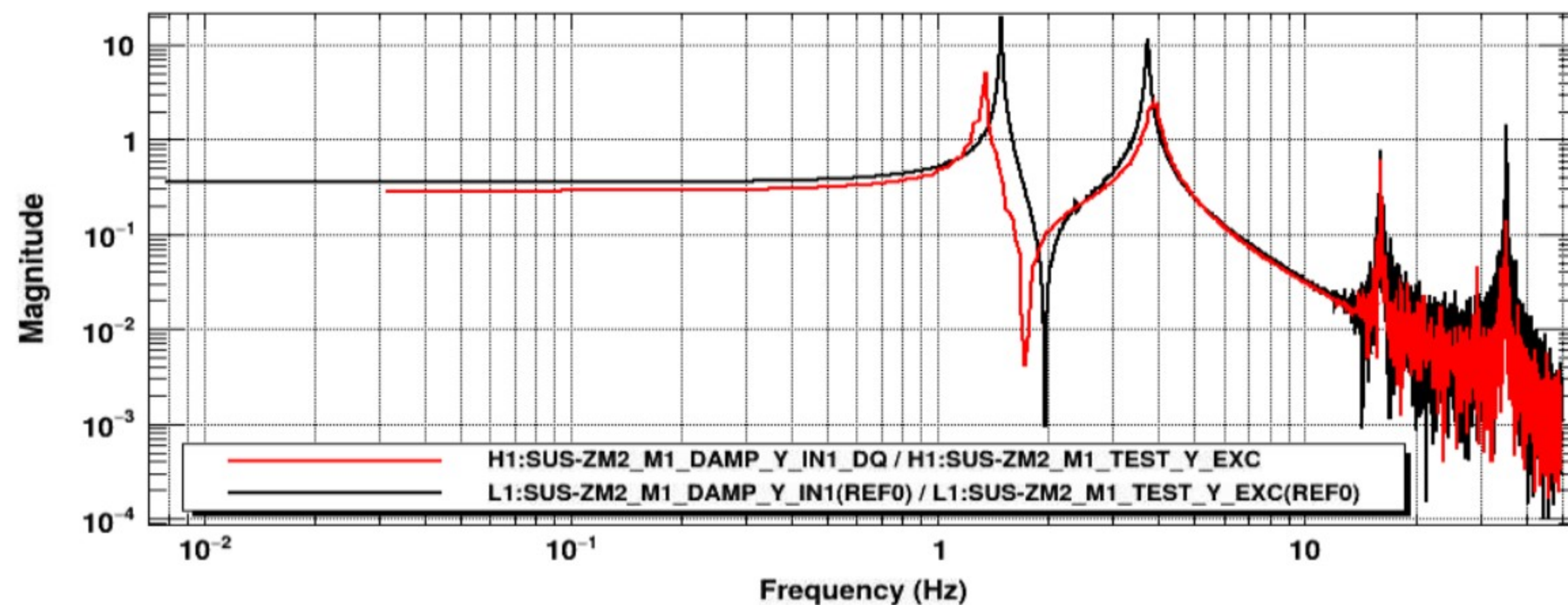
Transfer function
