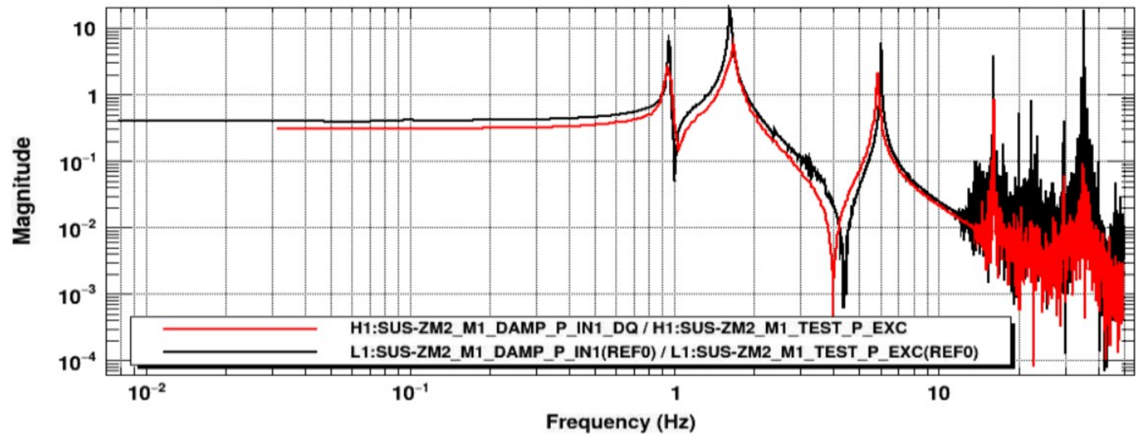
Transfer function
