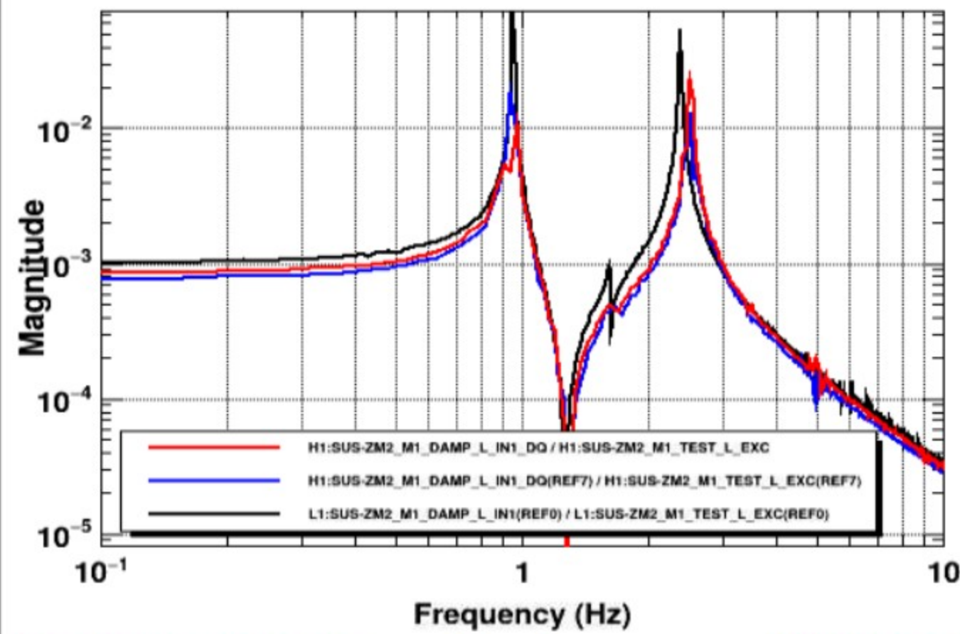
Transfer function
