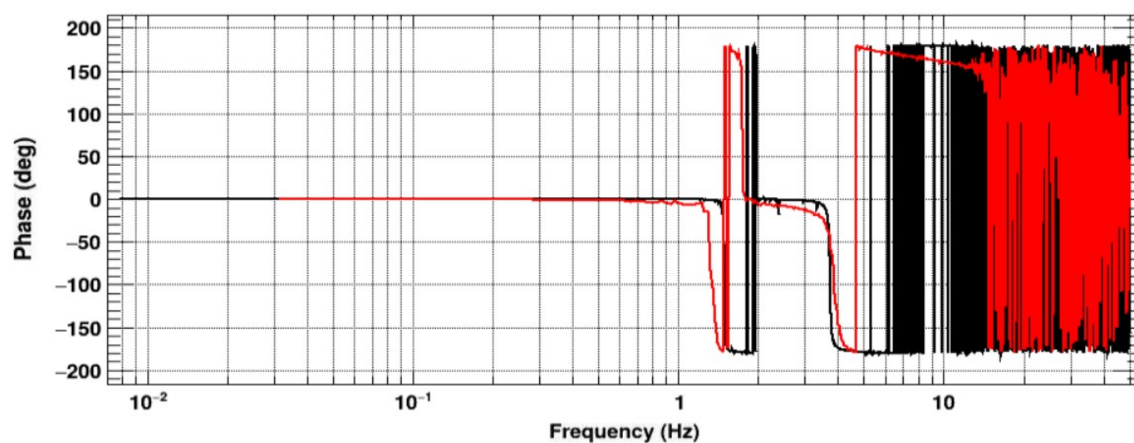
Transfer function
