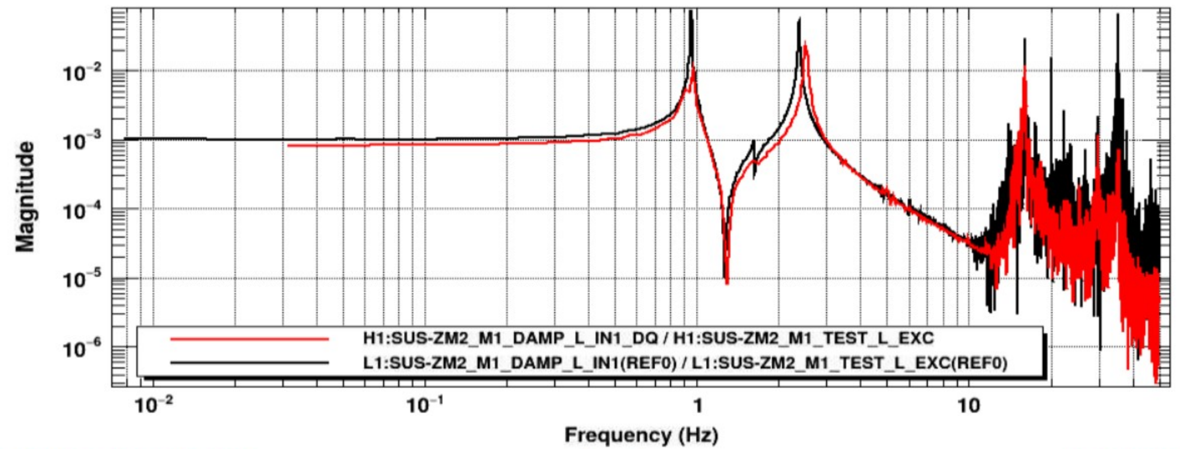
Transfer function
