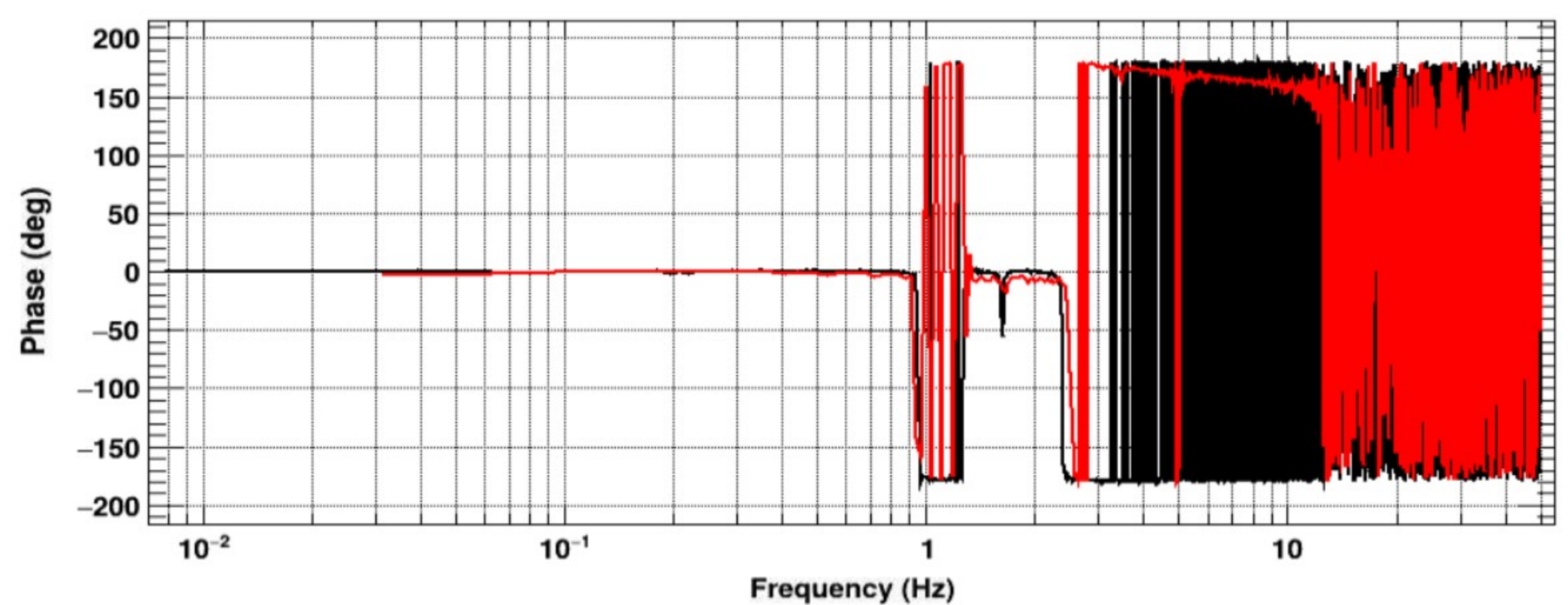
Transfer function
