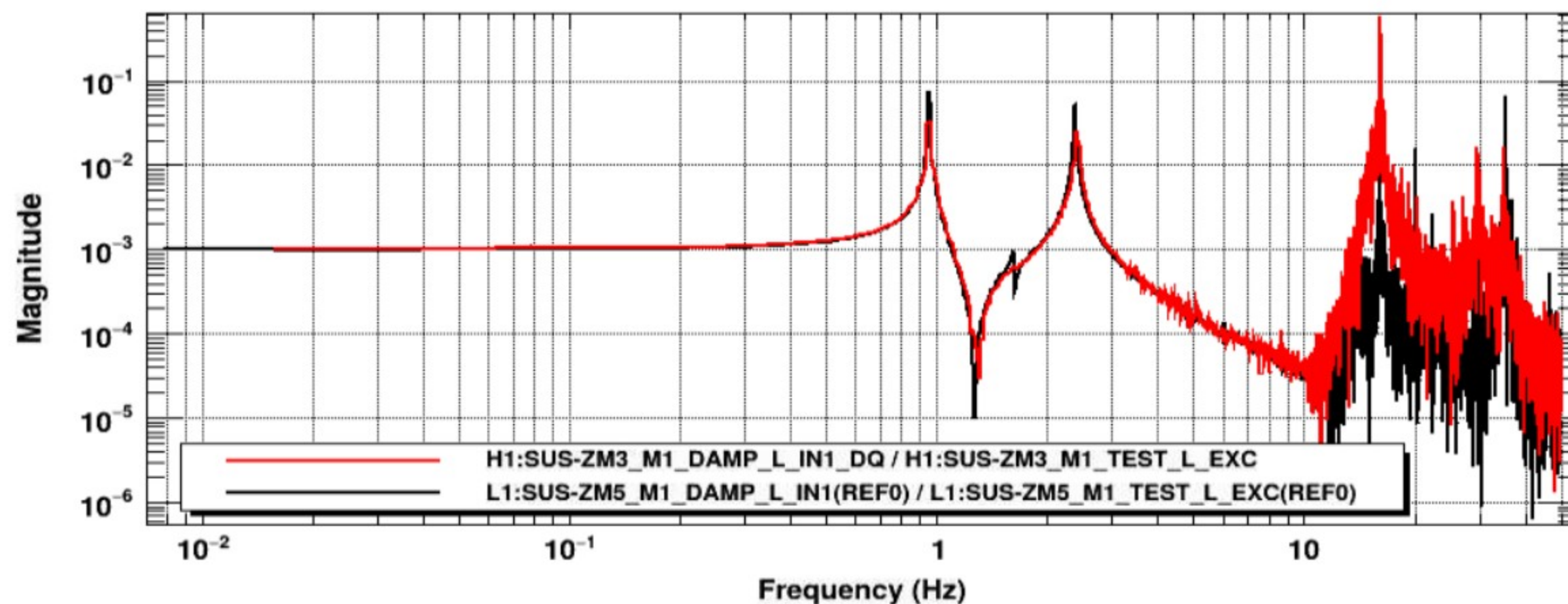
Transfer function
