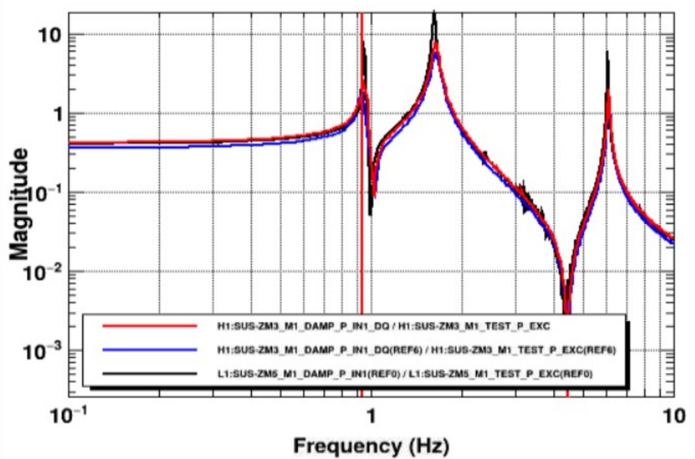
Transfer function
