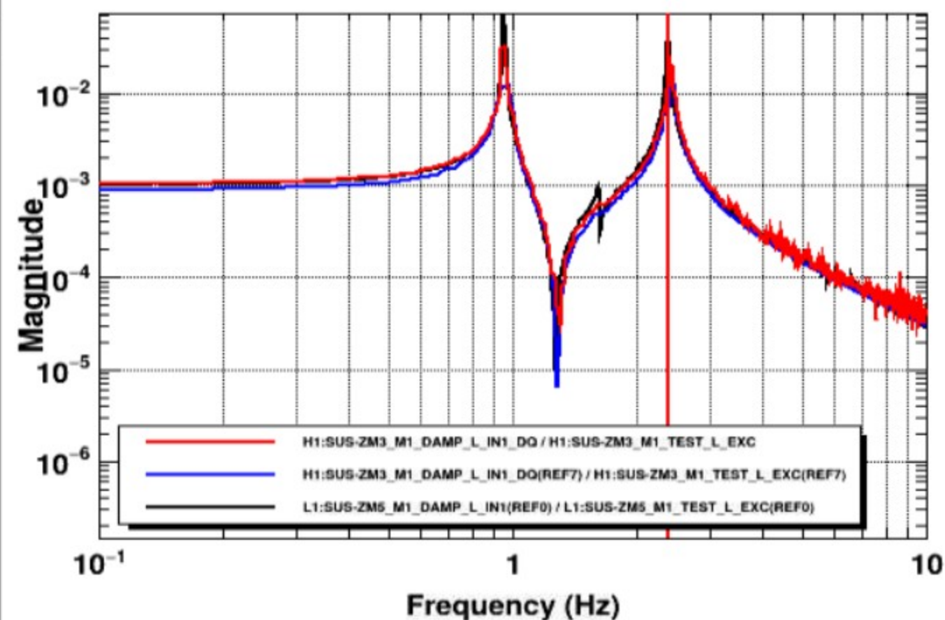
Transfer function
