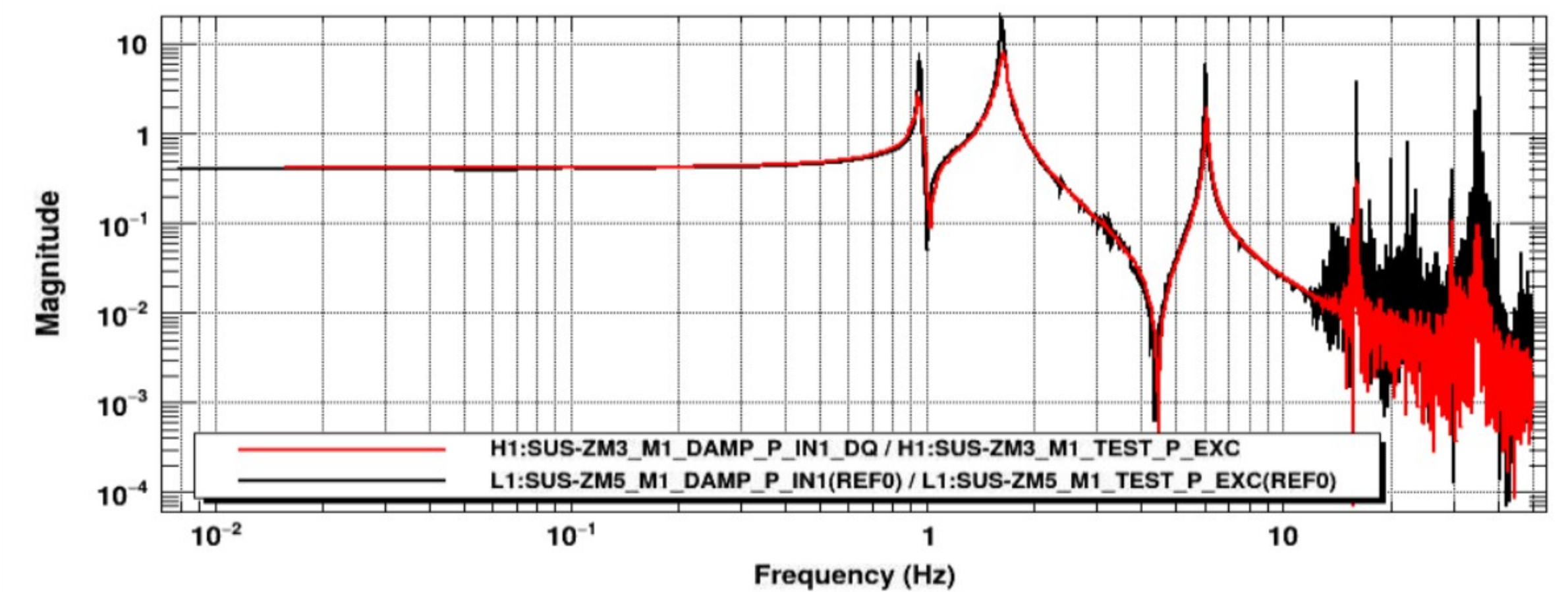
Transfer function
