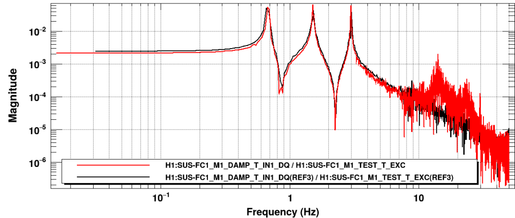
Transfer function
