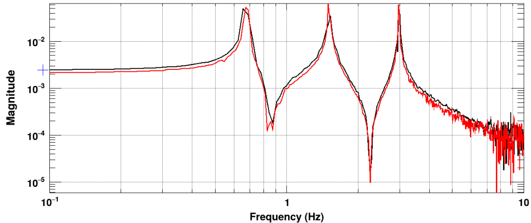
Transfer function
