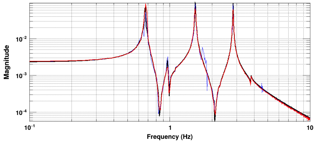
Transfer function
