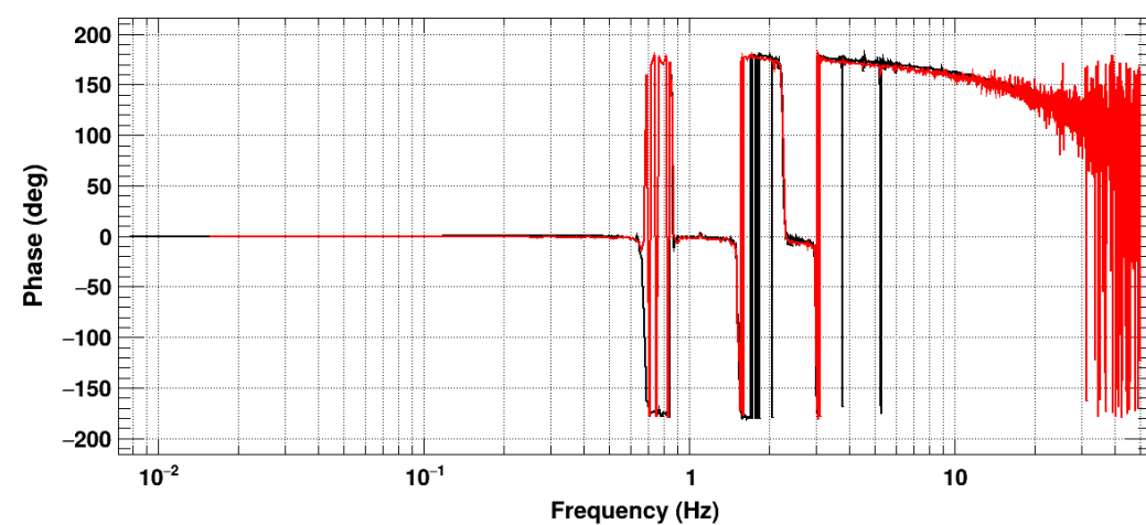
Transfer function
