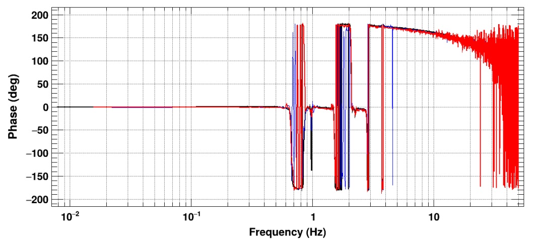
Transfer function
