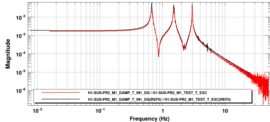
Transfer function
