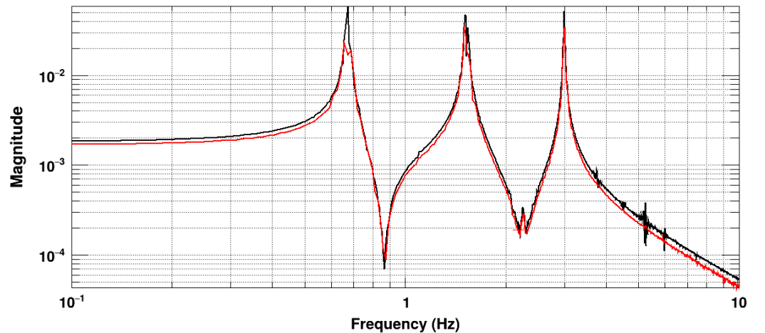
Transfer function
