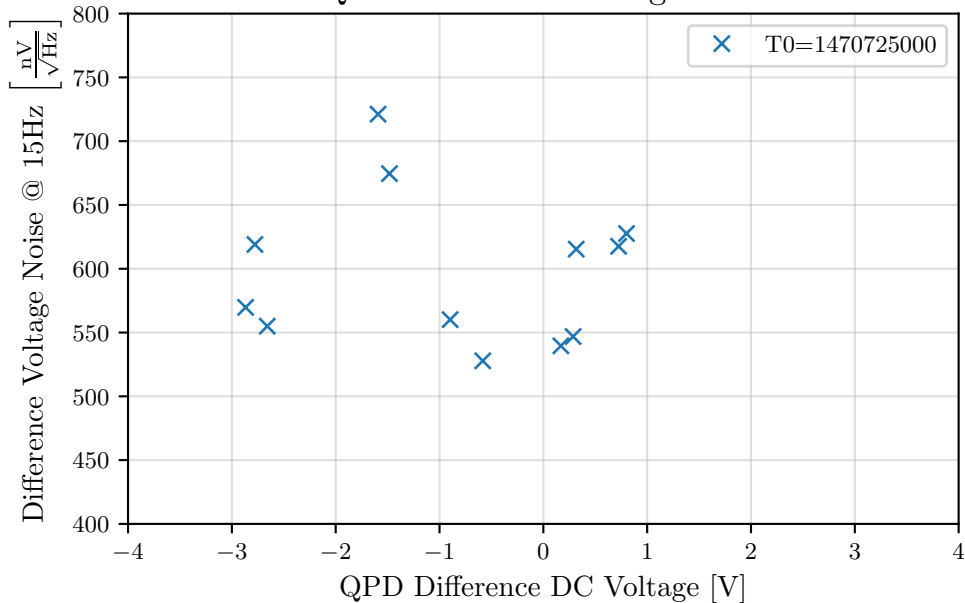
LHO BBSS QOSEM Difference Signal Offset vs Noise
