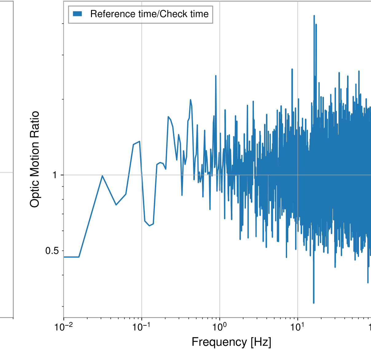
H1:SUS-MC3_M1_DAMP_V_IN1_DQ
