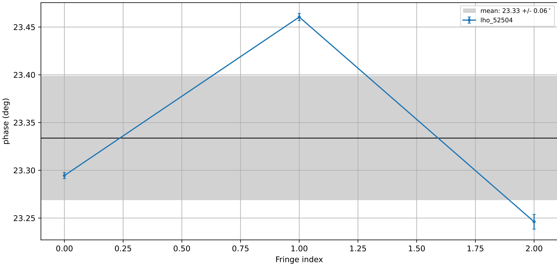
Single pass Gouy phase (LHO:52504)
