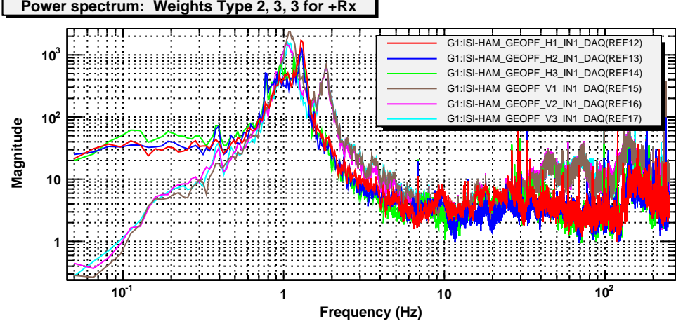
Power spectrum: Weights Type 2, 3, 3 for +Rx
