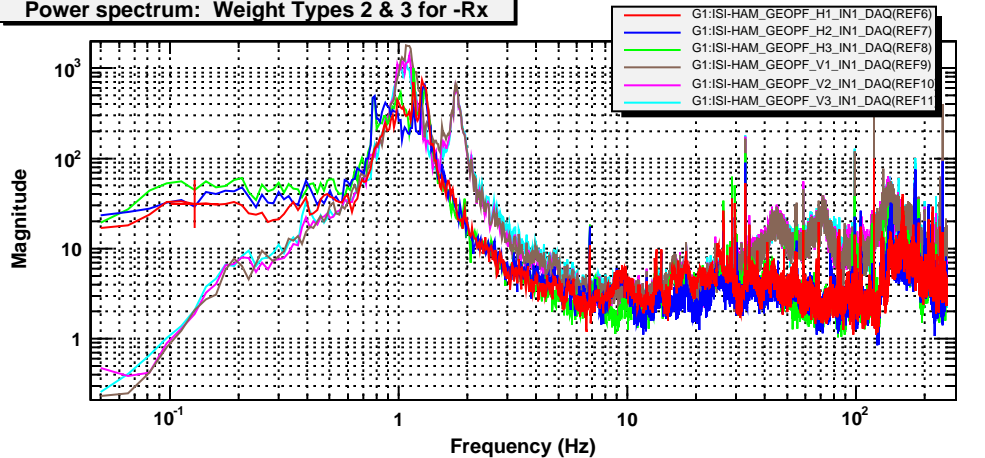
Power spectrum: Weight Types 2 & 3 for -Rx
