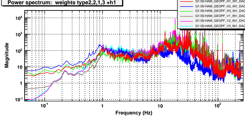
Power spectrum: weights type2,2,1,3 +h1
