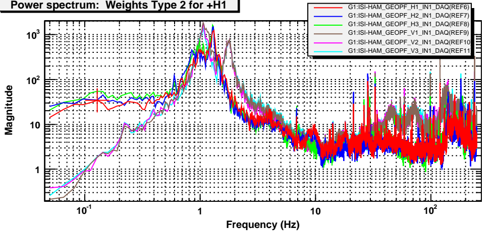
Power spectrum: Weights Type 2 for +H1
