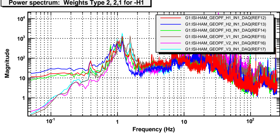
Power spectrum: Weights Type 2, 2,1 for -H1
