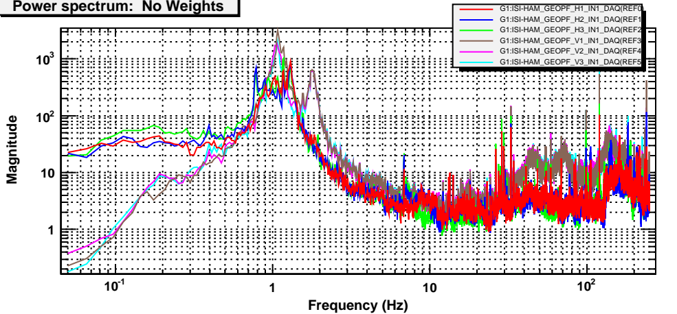
Power spectrum: No Weights
