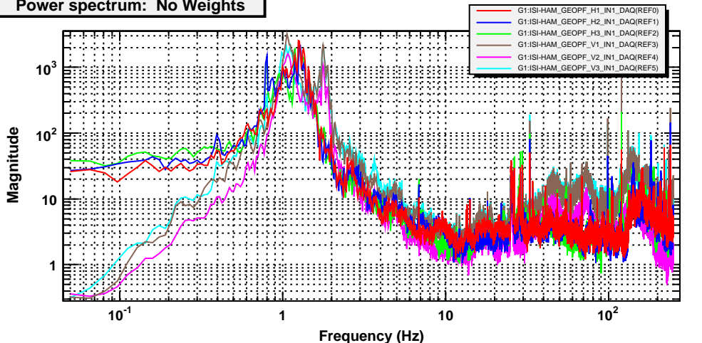
Power spectrum: No Weights
