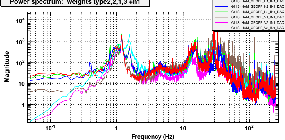
Power spectrum: weights type2,2,1,3 +h1
