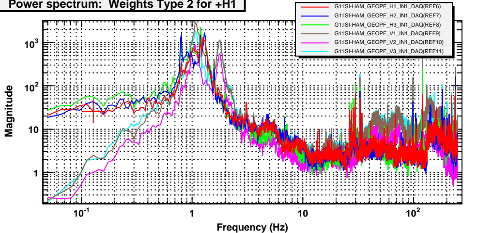
Power spectrum: Weights Type 2 for +H1
