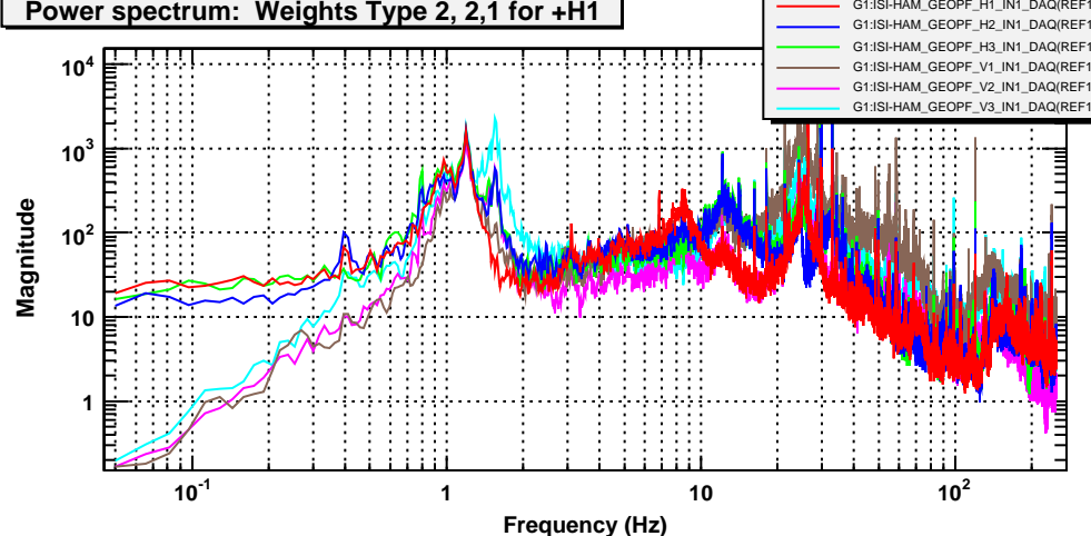
Power spectrum: Weights Type 2, 2,1 for +H1
