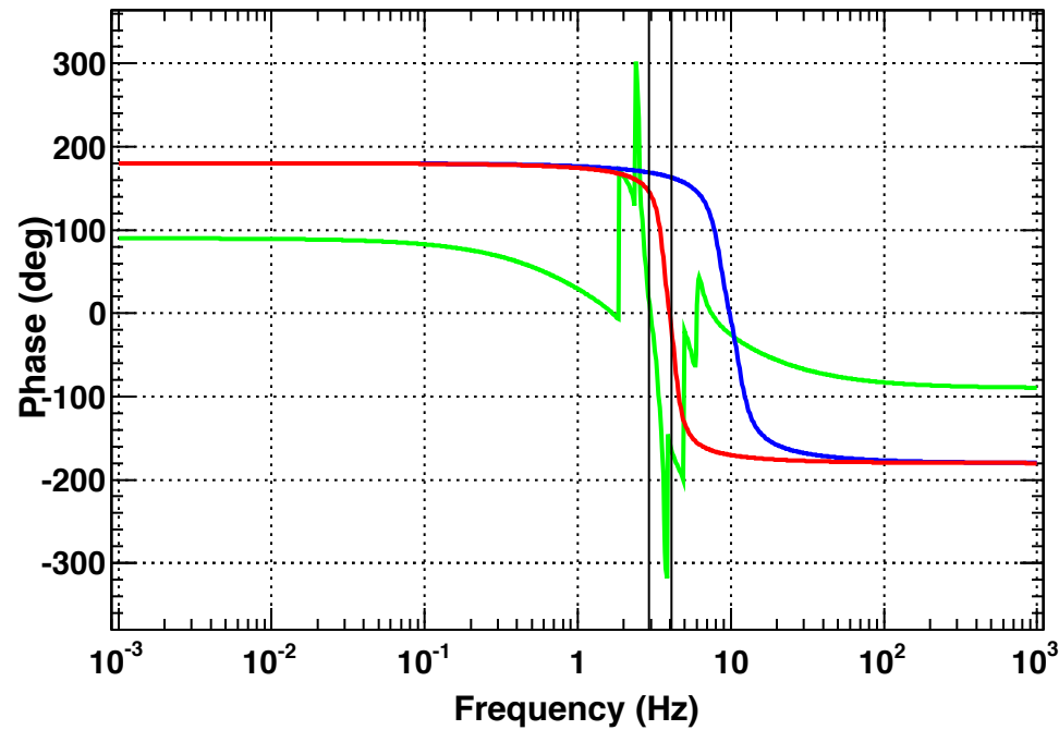
Transfer function
