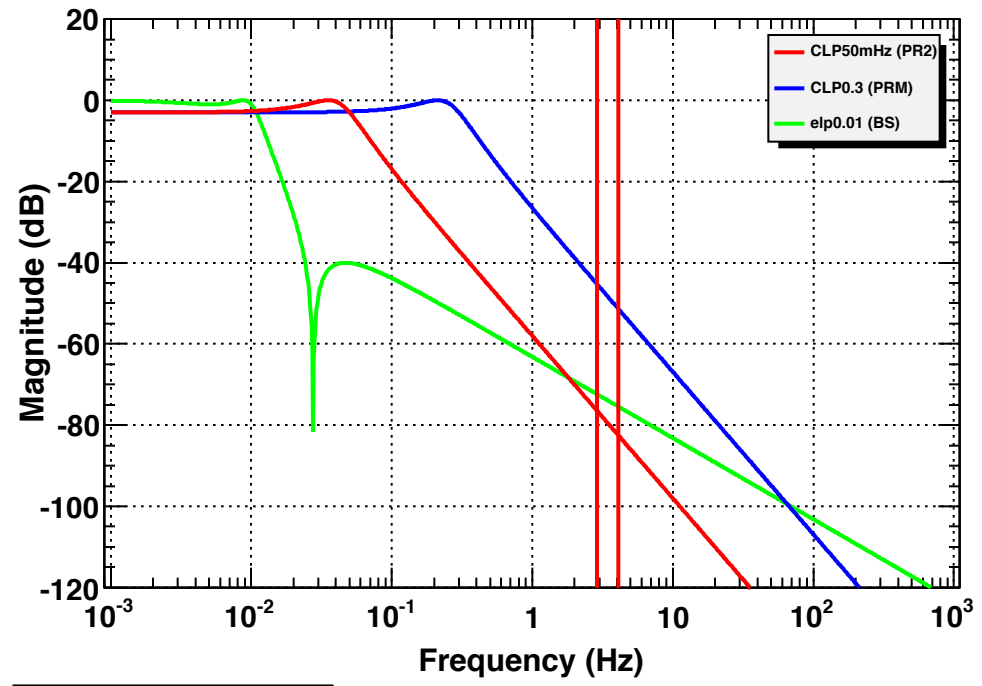
Transfer function
