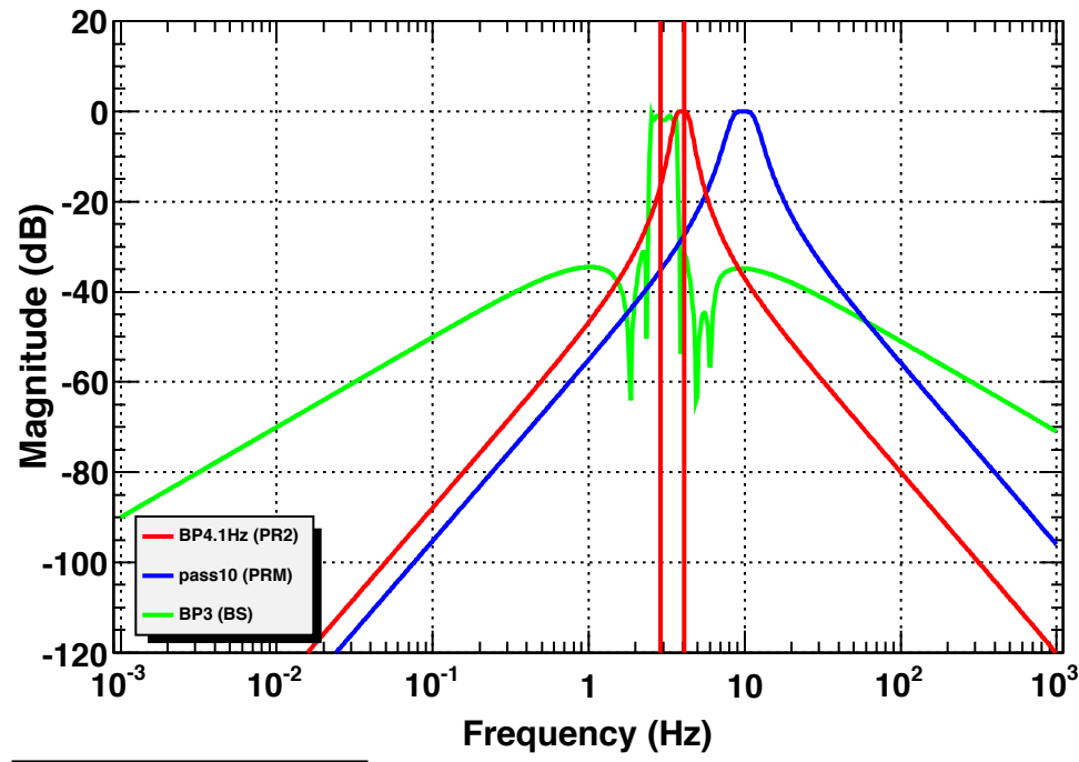
Transfer function
