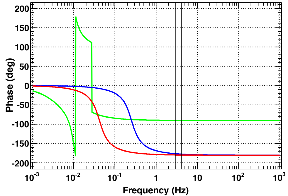
Transfer function
