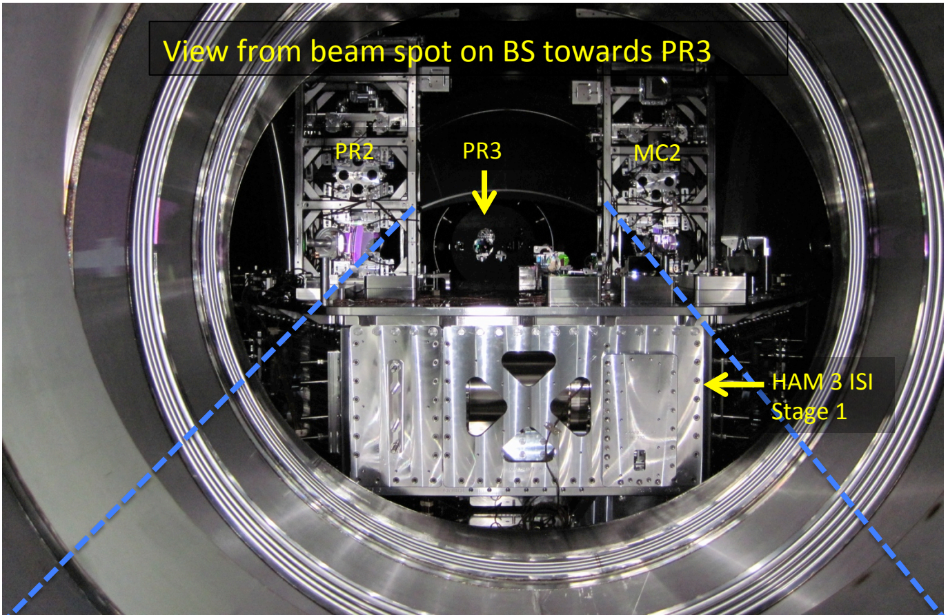
View from beam spot on BS towards PR3
