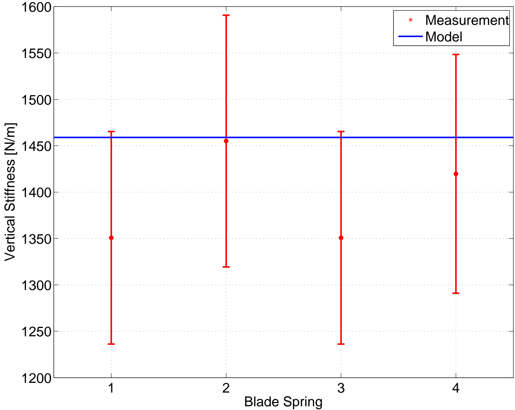
X1 BSFM M1 Spring Blade Vertical Stiffness
