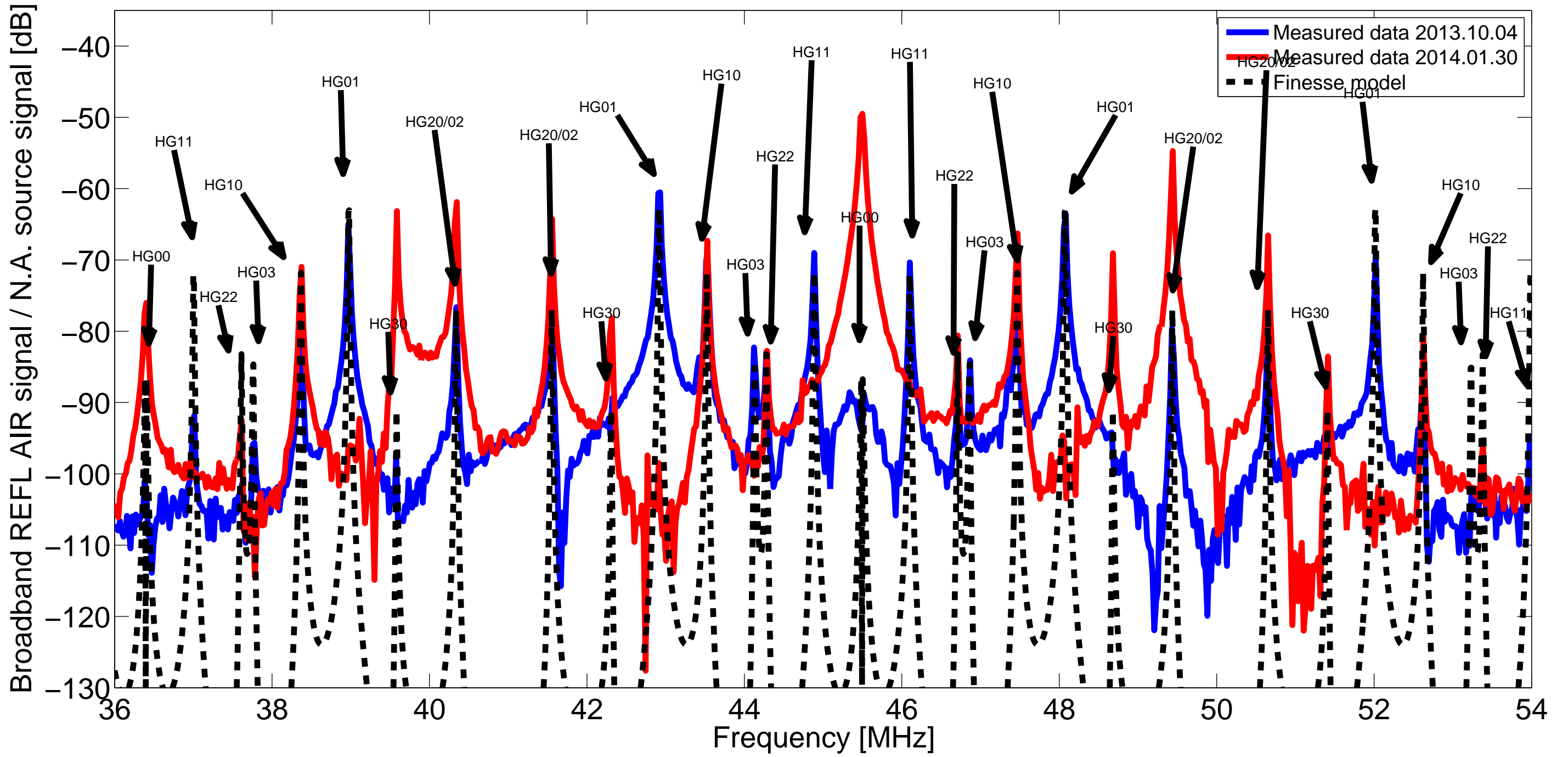
RF sideband sweep of H1 IMC Oct 2013 vs Jan 2014
