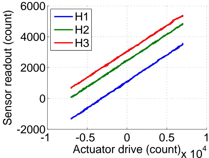
Stage 2 - Horizontal actuators to Horizontal CPS
