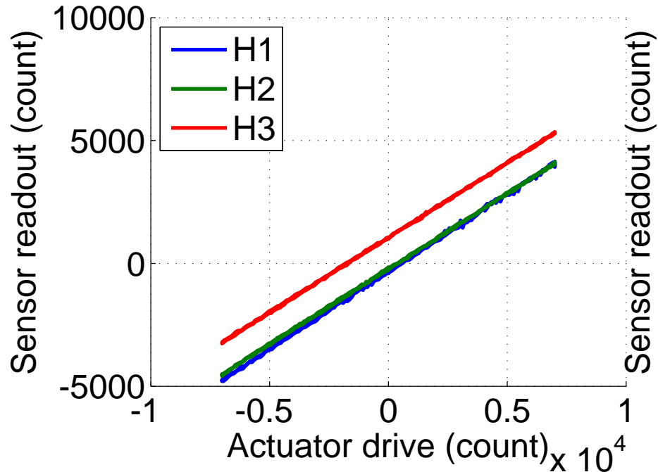
Stage 2 - Horizontal actuators to Horizontal CPS
