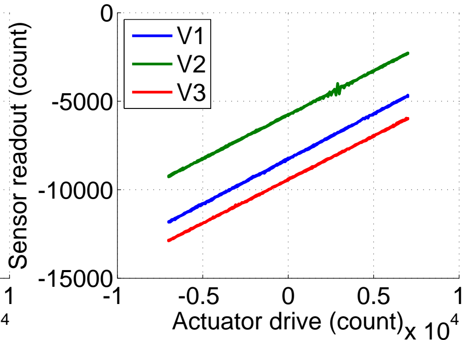
Stage 2 - Vertical actuators to Vertical CPS
