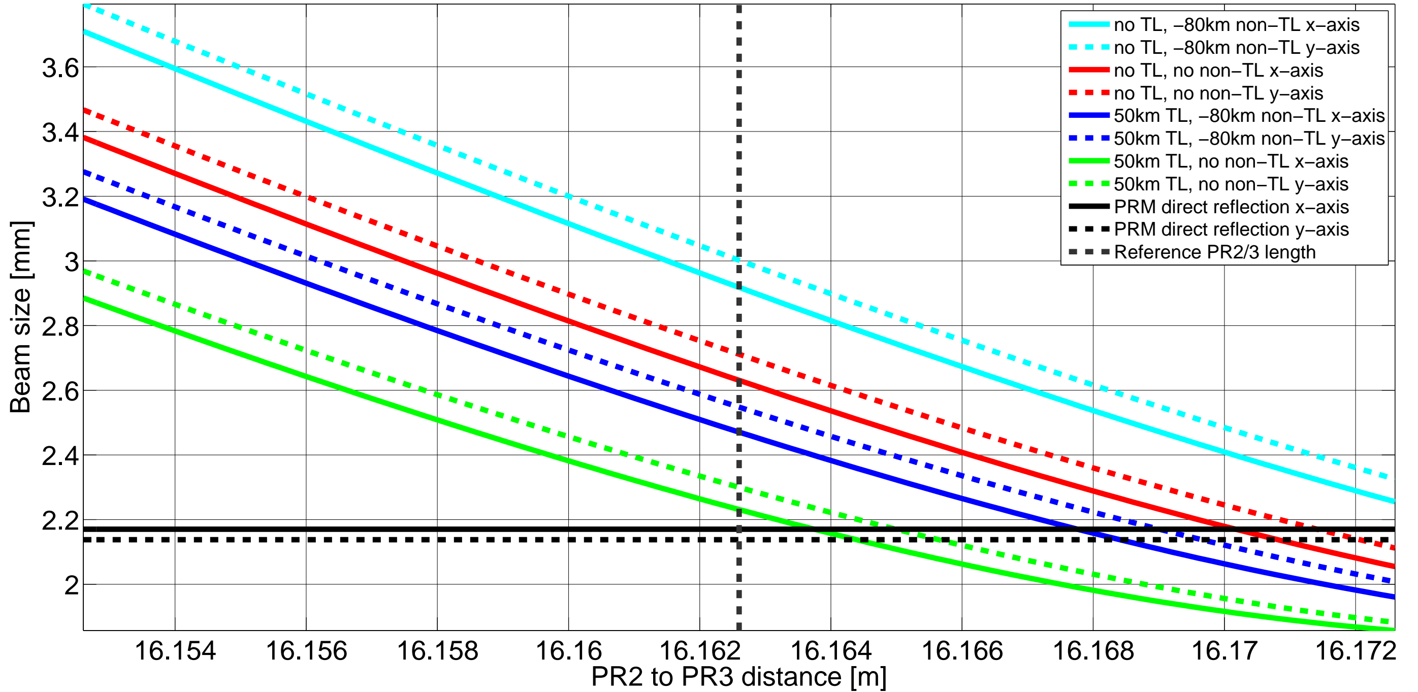
ITMX direct reflected beam sizes on ISCT1 before REFL1
