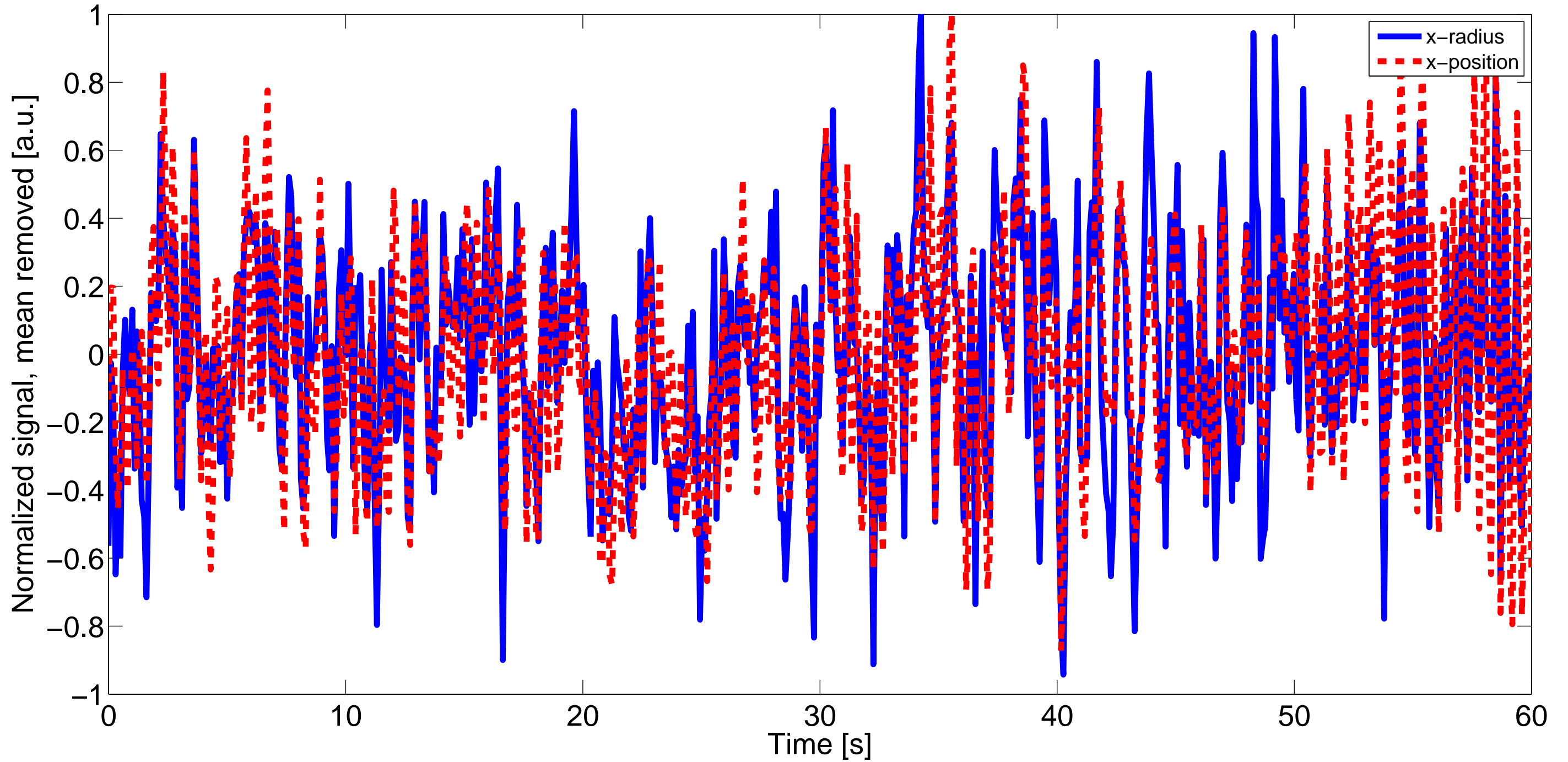
Beam radius and position data from nanoscan, ITMX direct reflected beam
