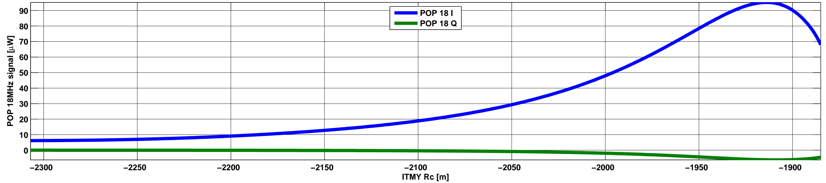
POP 18MHz sideband signal in H1 PRMI over ITMY Rc
